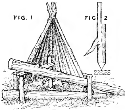
THE TURN TRIGGER.
