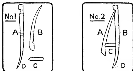
MARTEN TRAP TRIGGERS.
