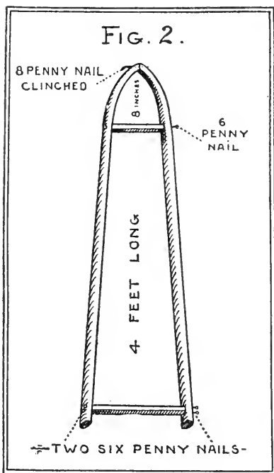
STRETCHING FRAME.
