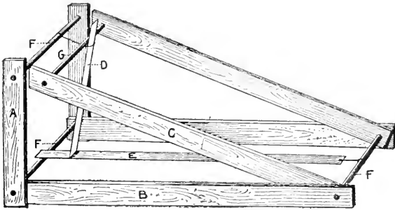
THE NOX-EM-ALL DEADFALL.
