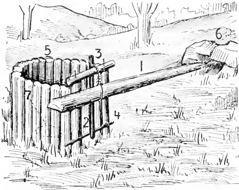
SMALL ANIMAL FALL.
