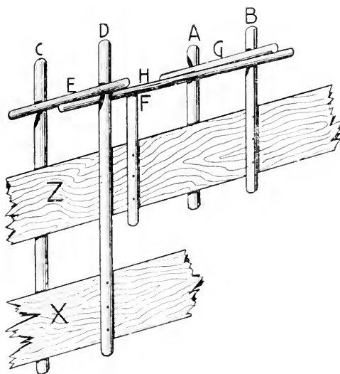
MARTEN DEADFALL.
