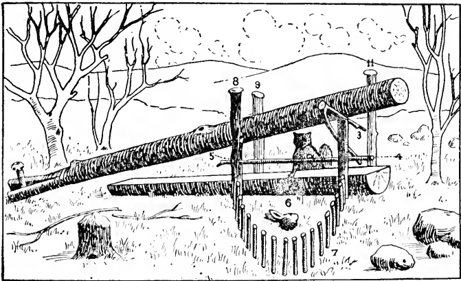
ANIMAL ENTERING TRIP DEADFALL.
