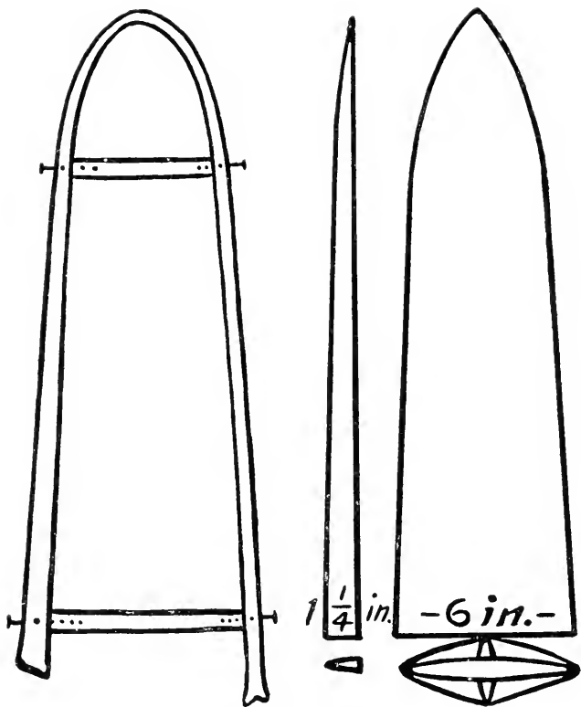
POLE STRETCHERS.
