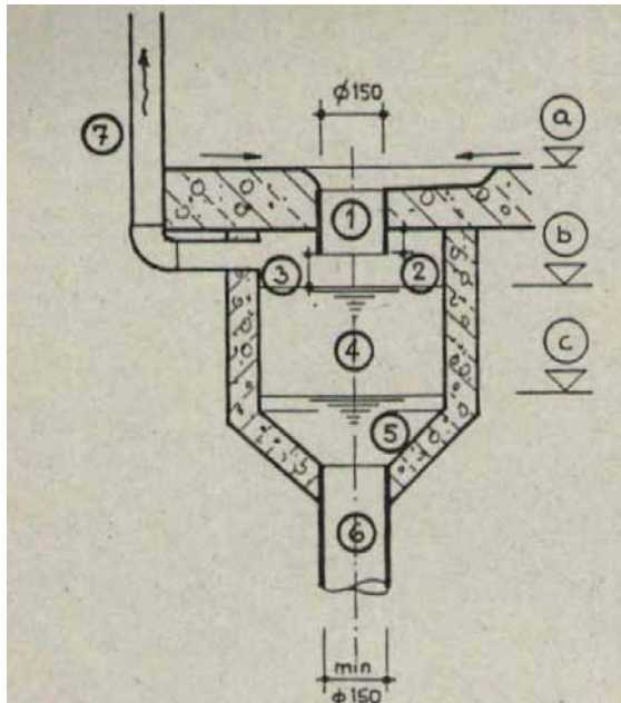
Fig. 8: Construction details of toilets for a biolatrine. [8]
