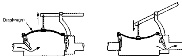
Figure 4: Diaphragm pump
