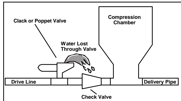
Figure 5. Ram Pump Components
