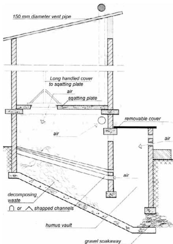
Fig. 6: Continuous composting toilet, „Multrum“-design. [1], p. 19
