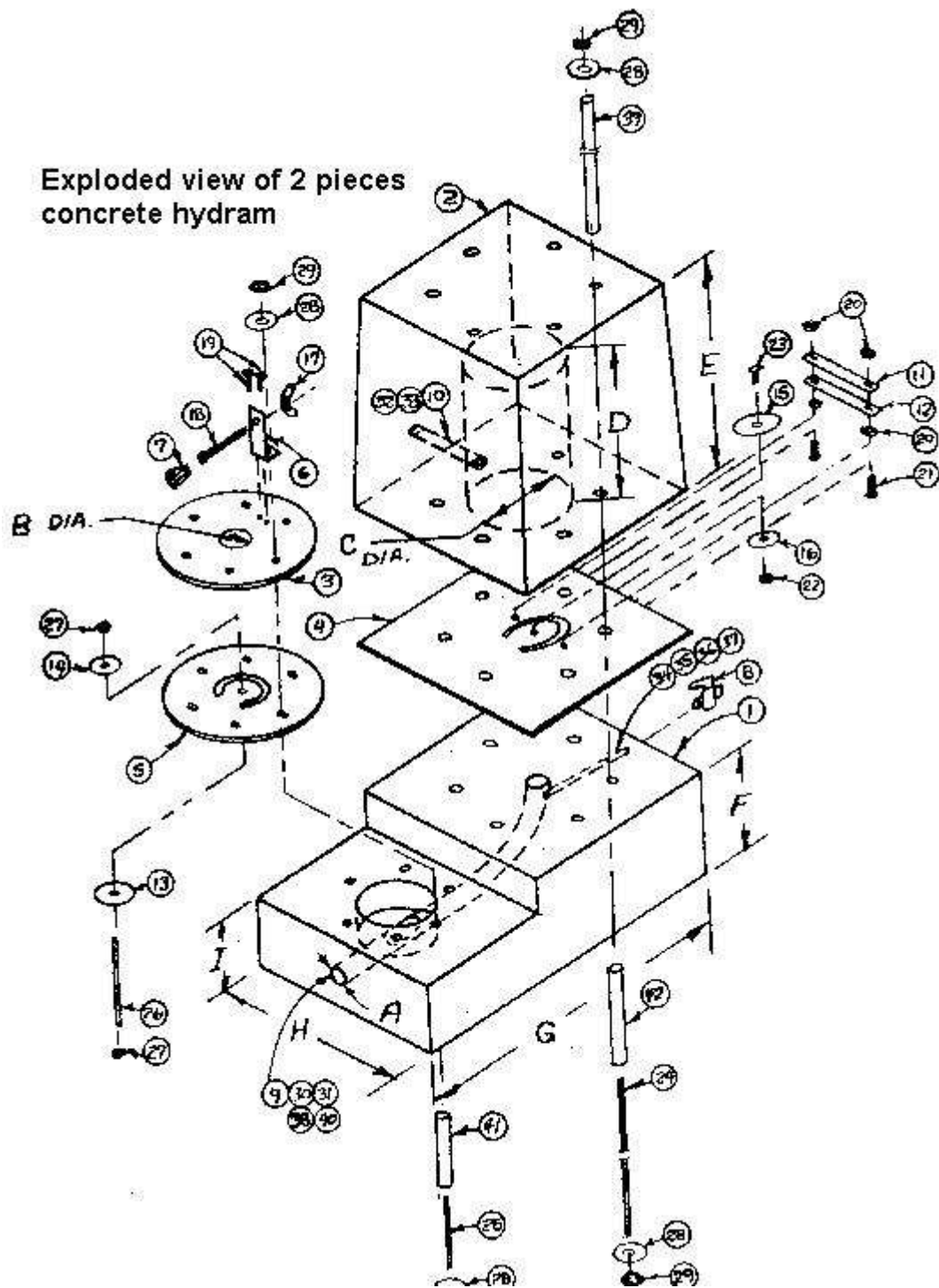
Exploded view of 2 piece concrete hydram
