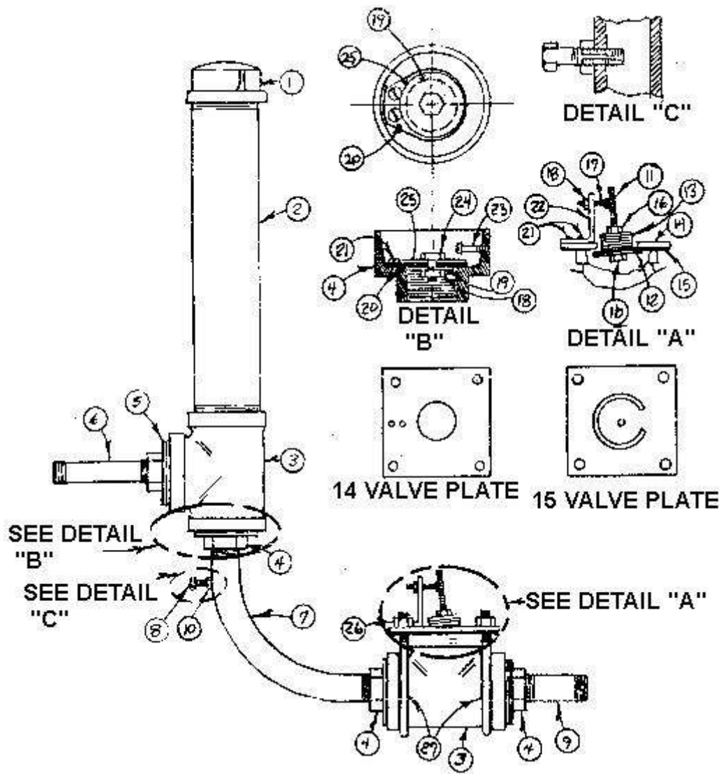
Pipe fitting hydram with field-made valves
