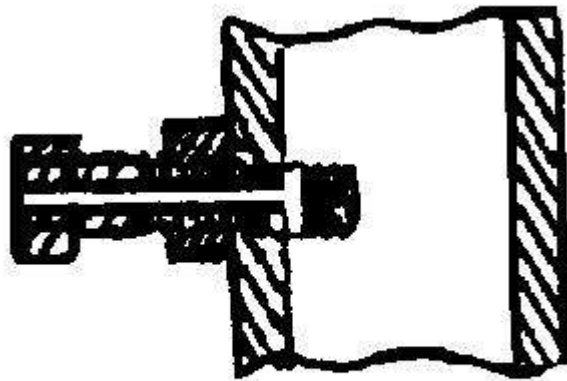
external drilled bolt snifter
