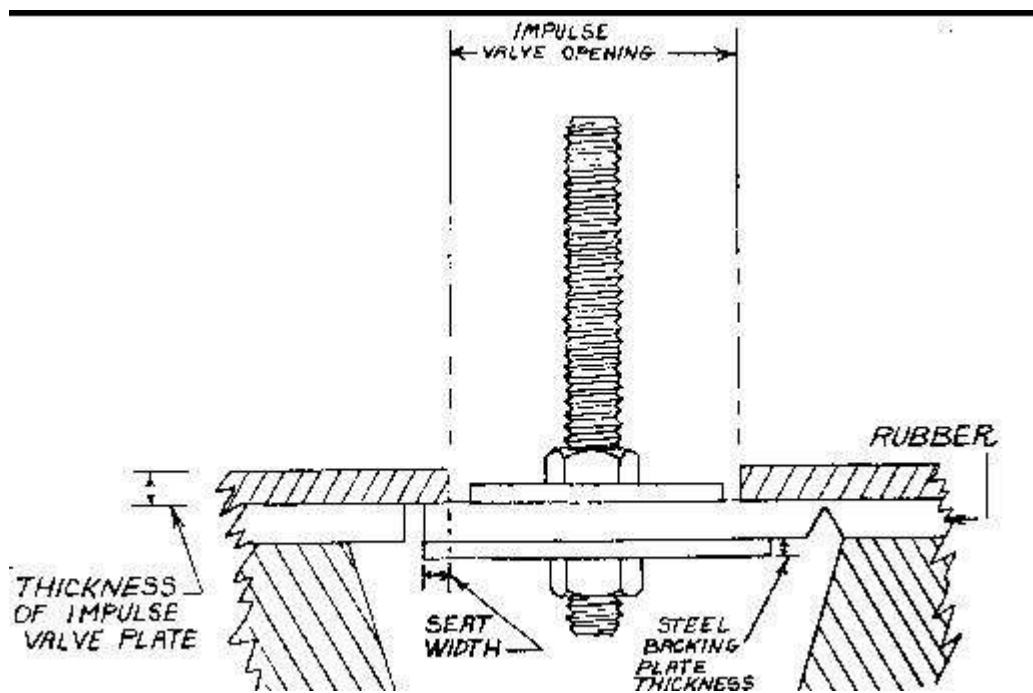
Impulse valve opening in inches
