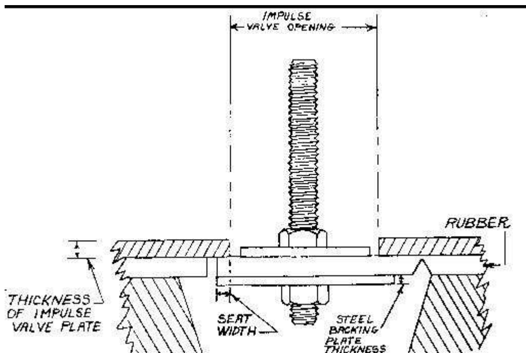
Thickness of the impulse valve plate in inches
