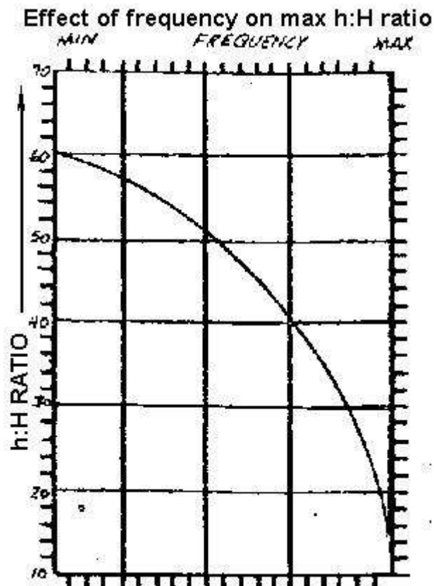
Effect of frequency on max h:H ratio
