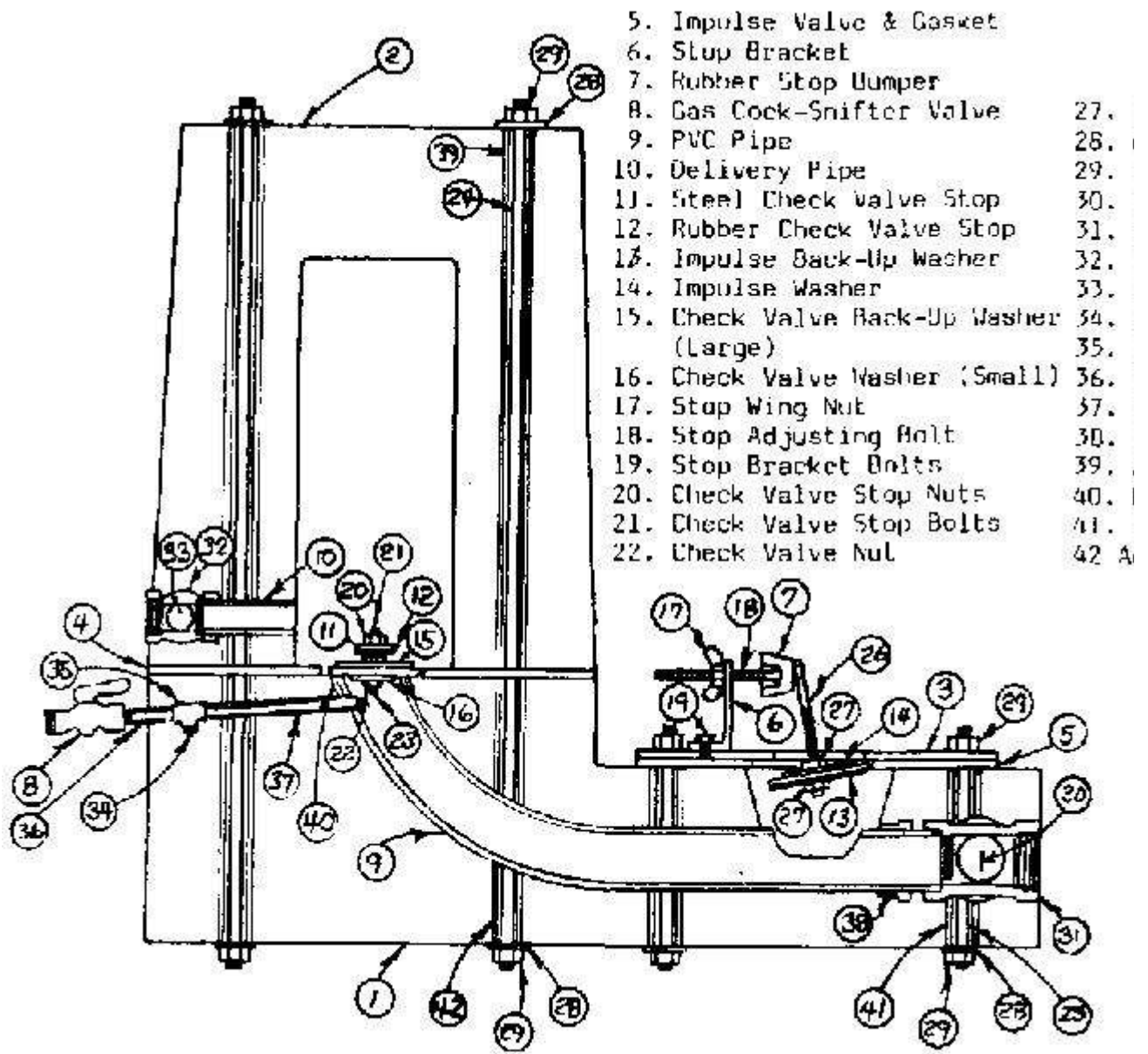
Exploded view of 2 - piece concrete hydram
