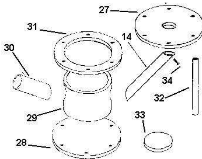
Welded hydam, impulse cavity: exploded view
