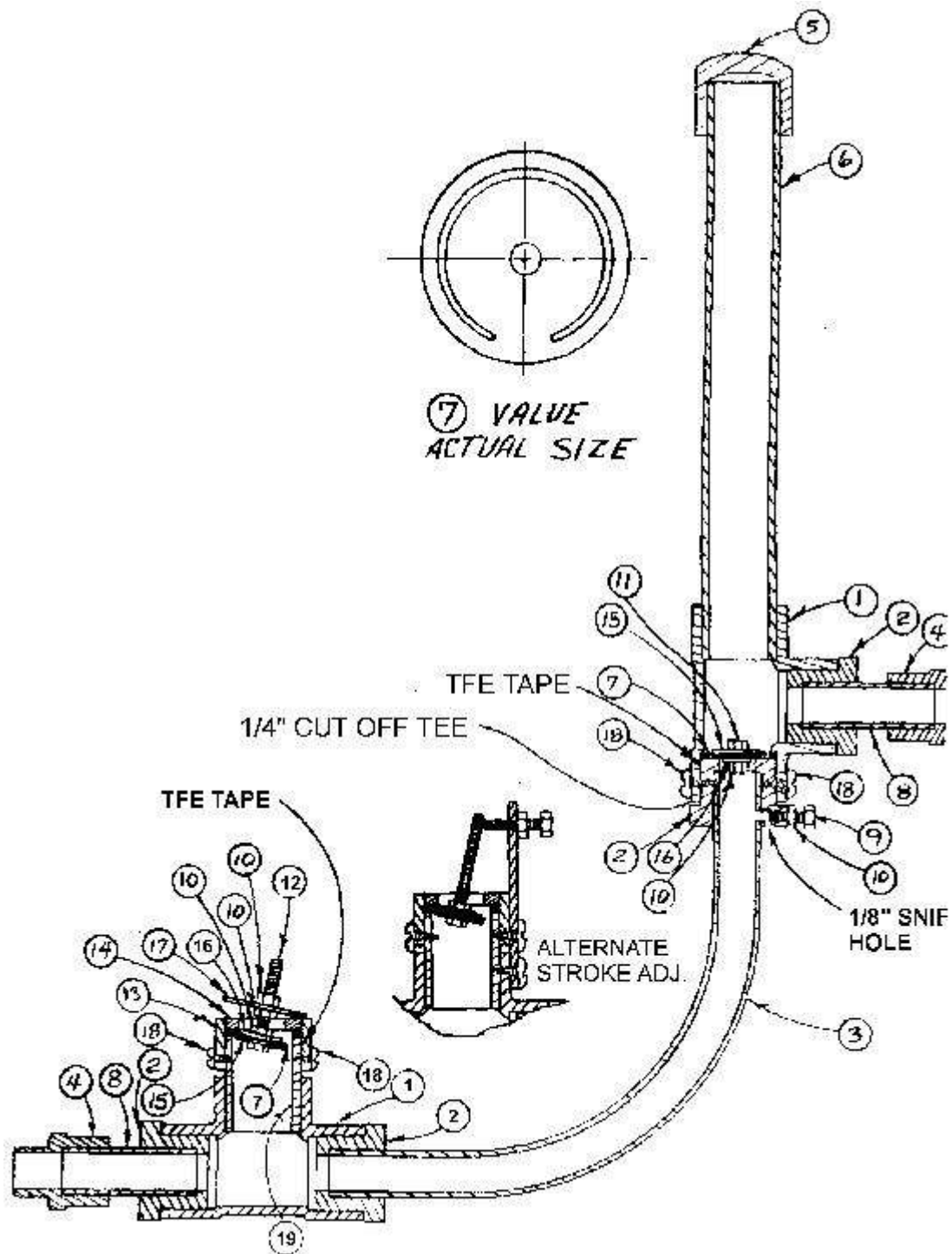
A PVC Hydram
