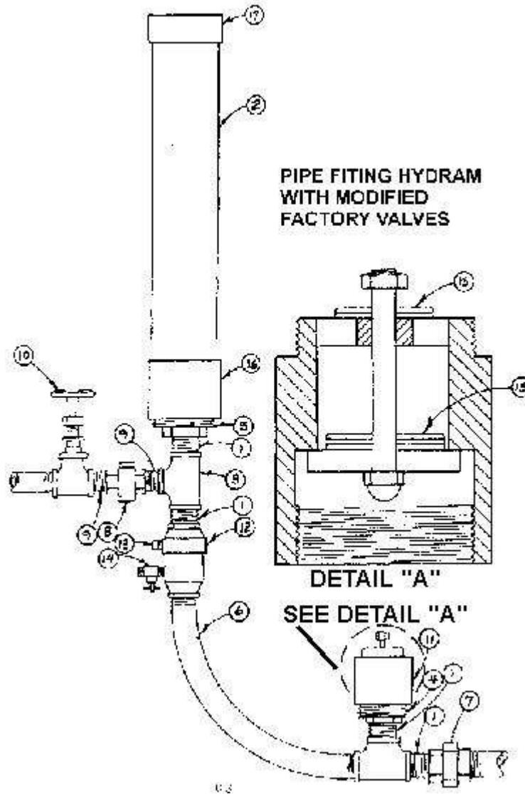
Pipe fitting hydam with modified factory valves
