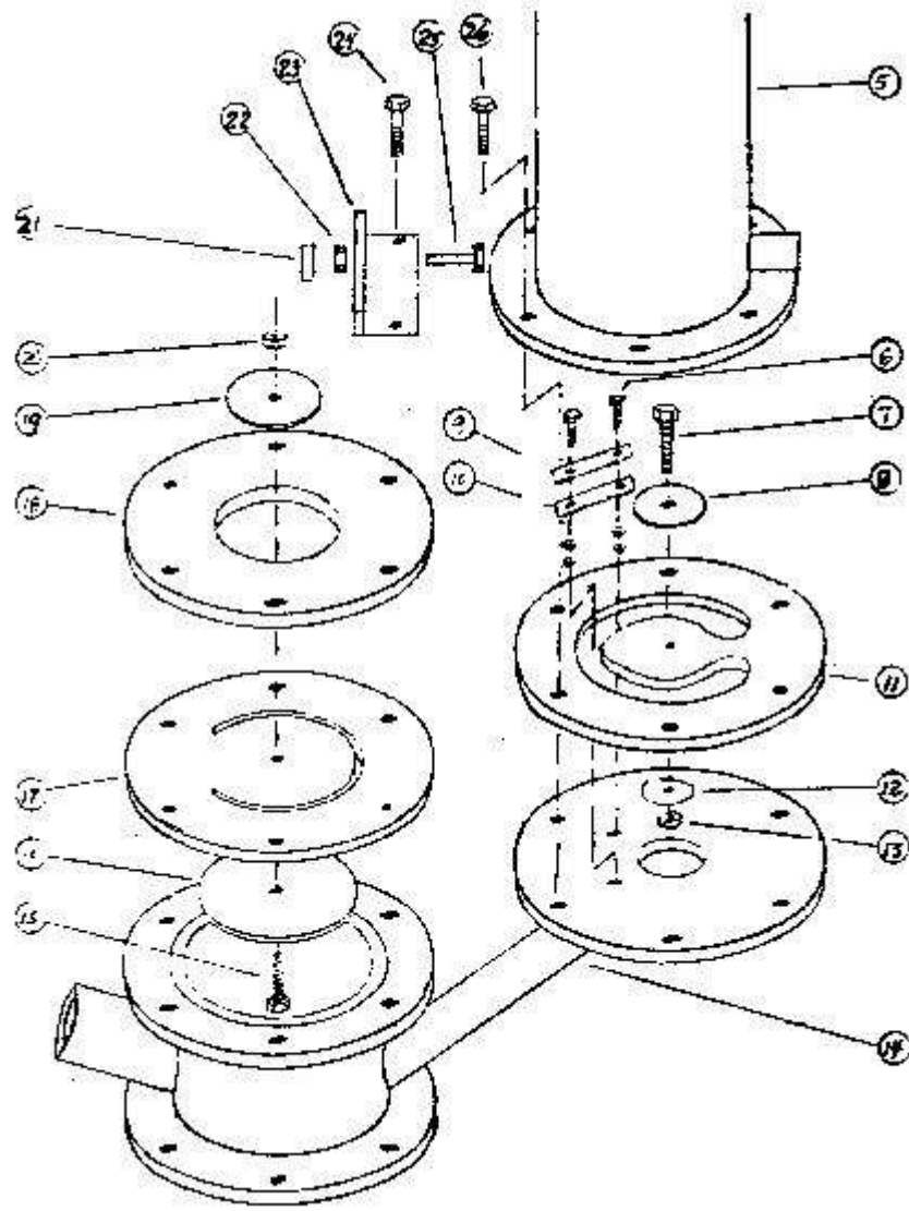
Welded hydram: exploded view
