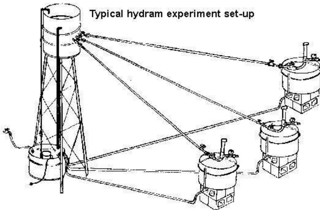
TYPICAL HYDRAM EXPERIMENT SET-UP
