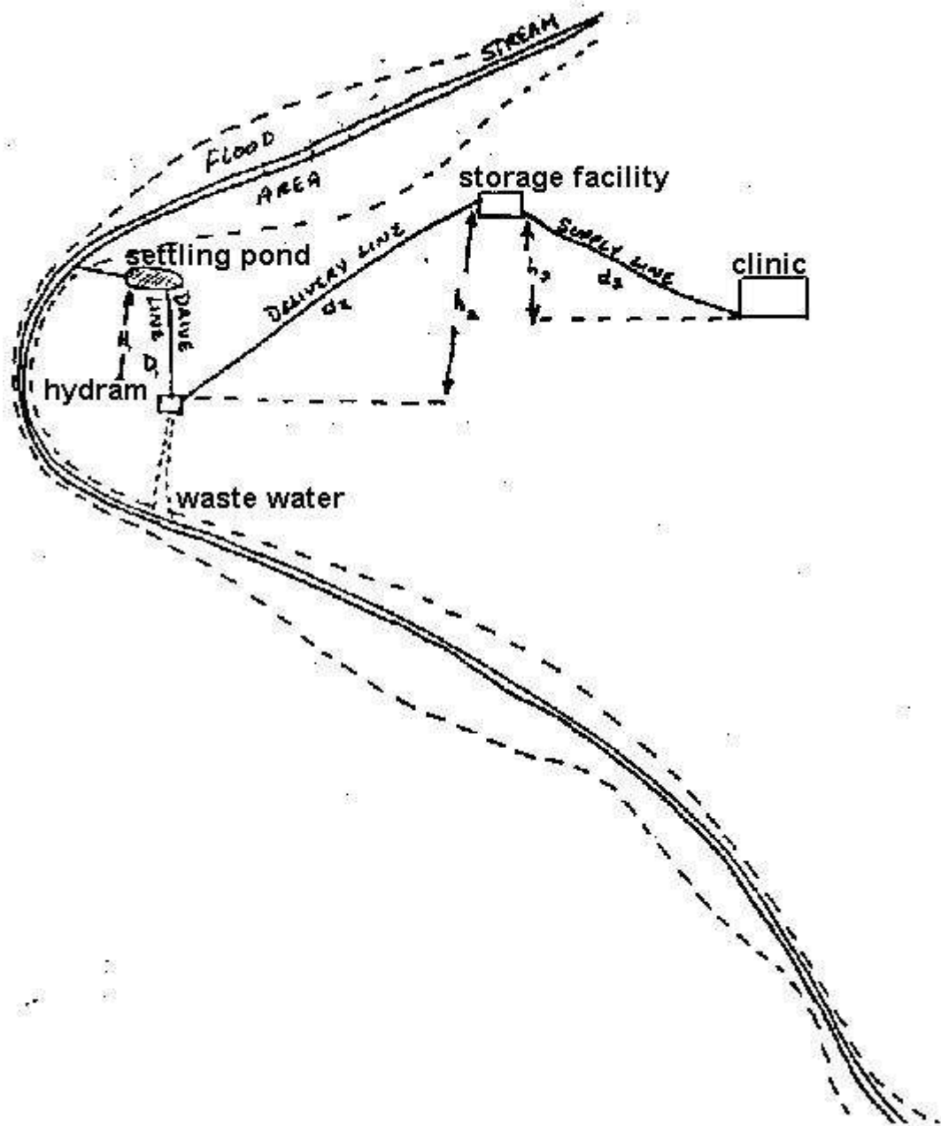
Diagram of hydam system for site selection
