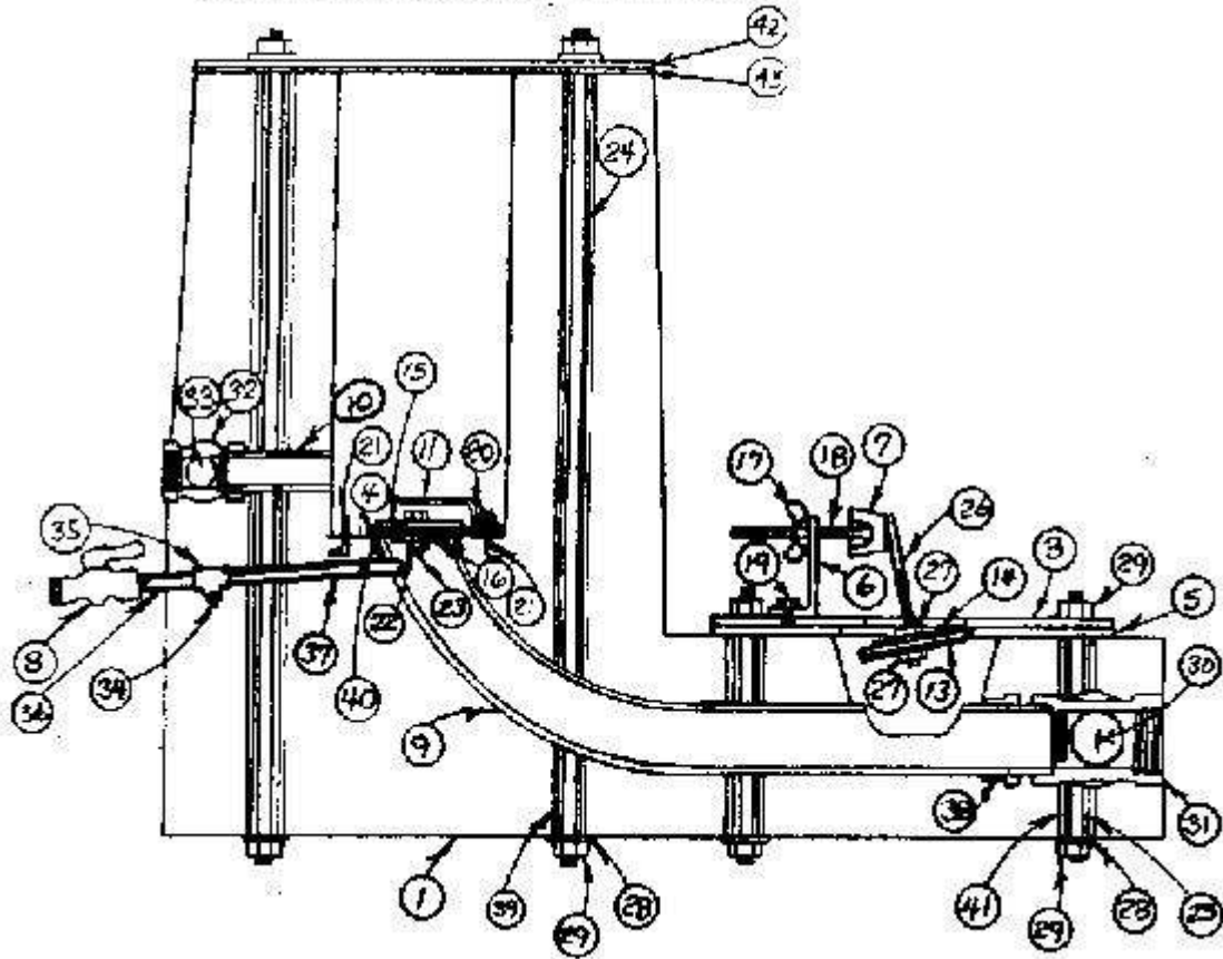
One-piece concrete hydram
