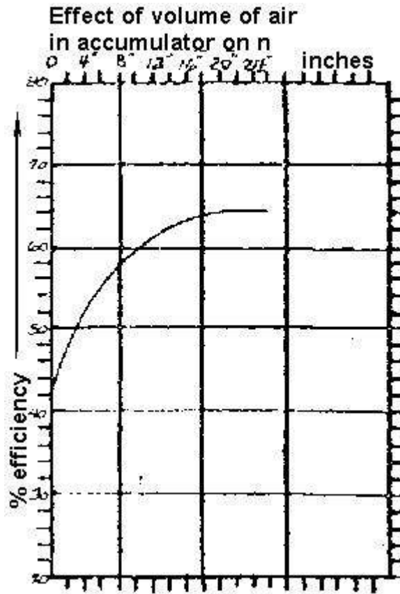
Effect of volume of air in accumulator on n
