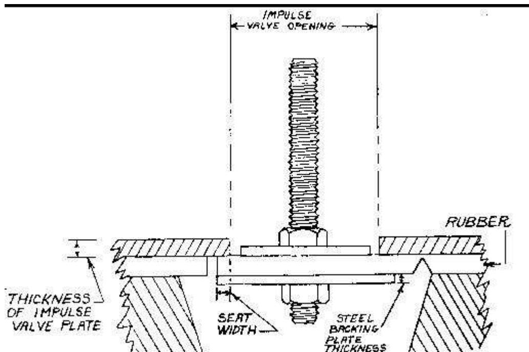
Impulse valve opening in millimeters
