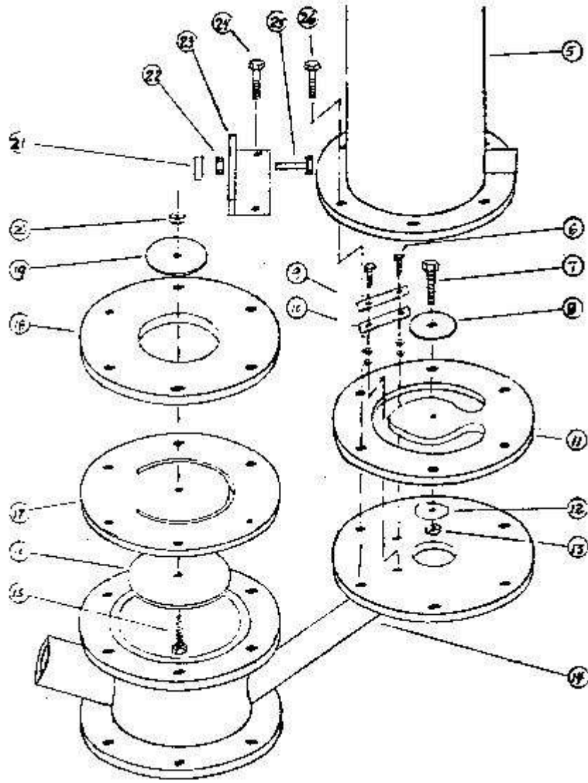
Welded hydam: exploded view
