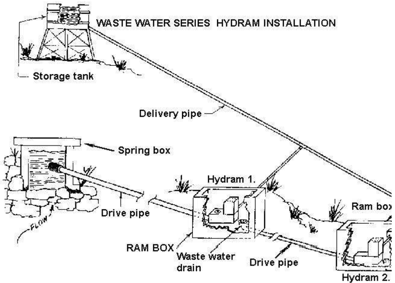
Waste water series hydam installation
