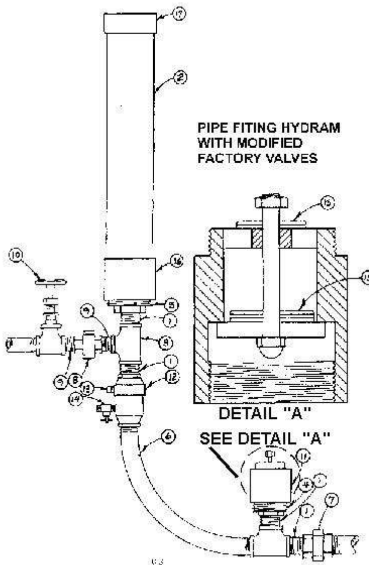
Pipefitting hydram with modified factory valves
