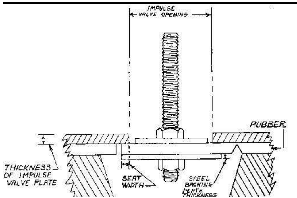
Impulse valve steel backing - metric
