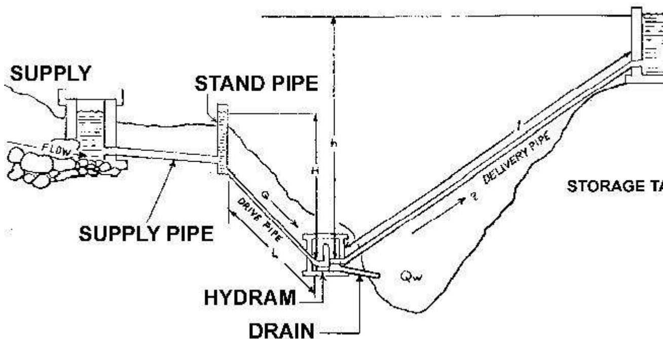
Hydram installation
