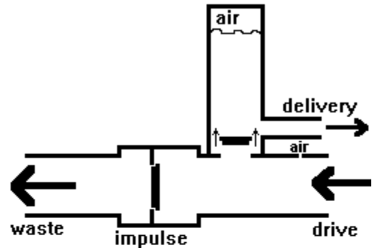
Figure 1b Compression
