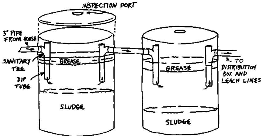
Details of two tank septic system.
