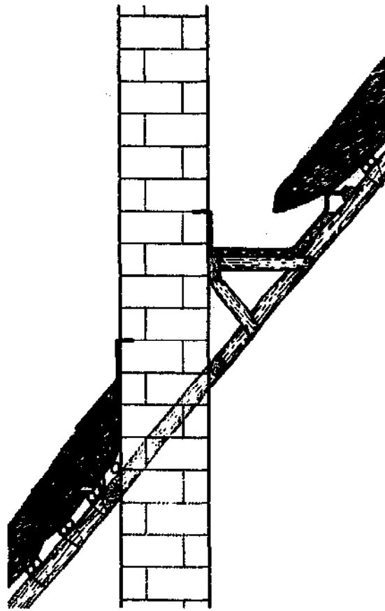
Fig. 3:8 Back-gutter behind chimney.
