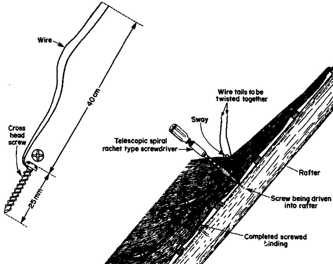
Fig. 4:5 Screwed binding.
