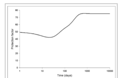
The protection factor provided by 20 cm of concrete shielding where the source is the idealised Chernobyl fallout. [23]
