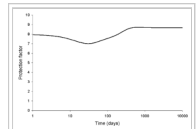
The protection factor provided by 10 cm of concrete shielding where the source is the idealised Chernobyl fallout. [23]
