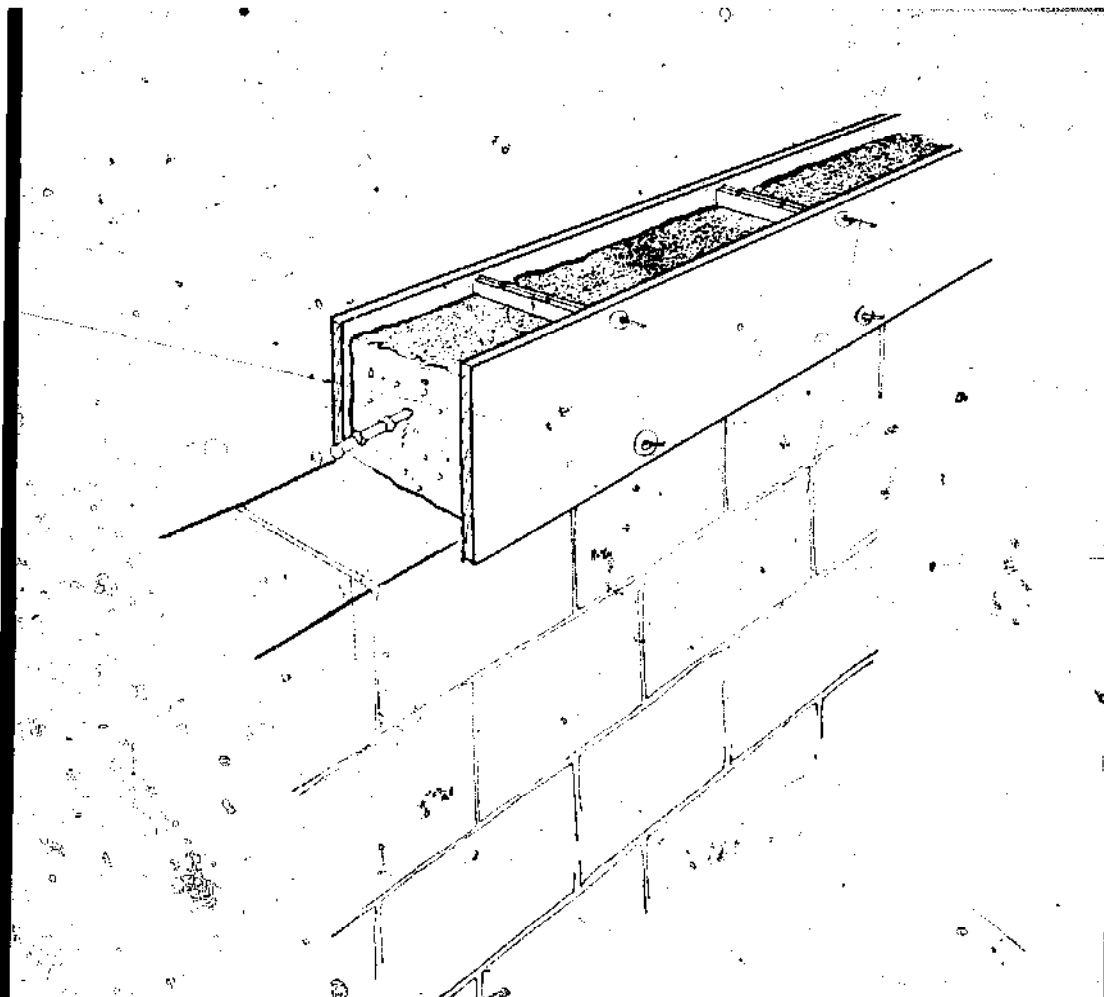
Figure 71. Forms like this can be used to pour concrete bond beams and lintels in place in the wall.
