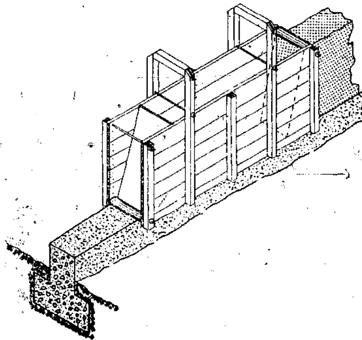
Figure 77. Form for ramming.
