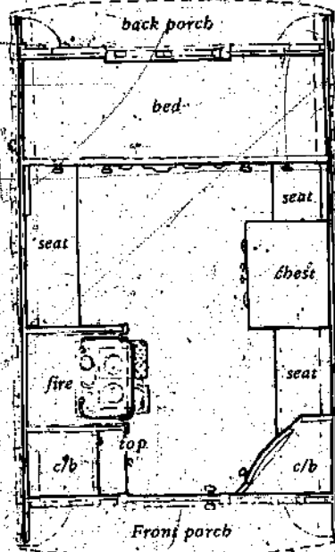
Plan
