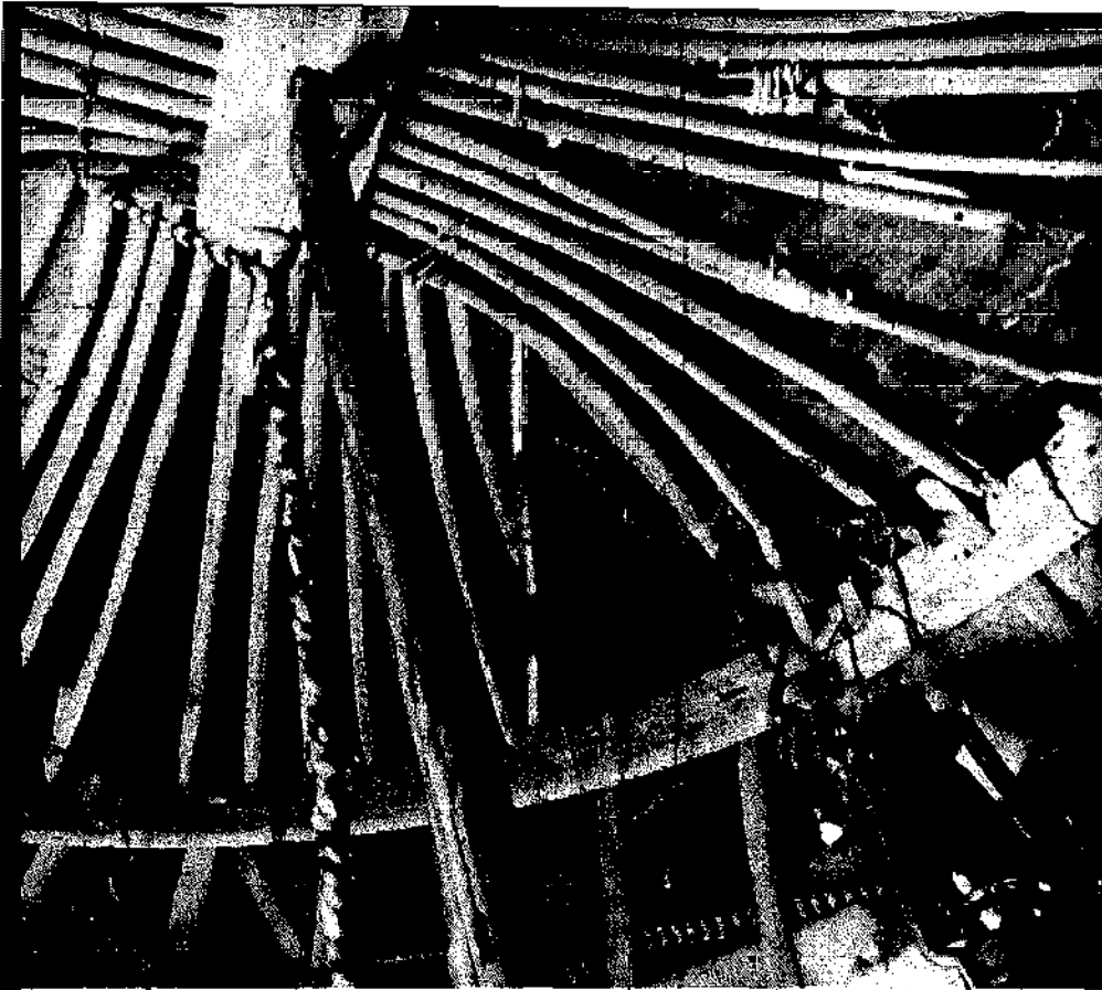
Topak ev type alaciks are prestressed structures: vertical tensioning is provided by a central post supporting the weight of the roof (dognuk) and a rope tie-down for wind uplift. Flat curved sticks radiating from center are ug sticks.
