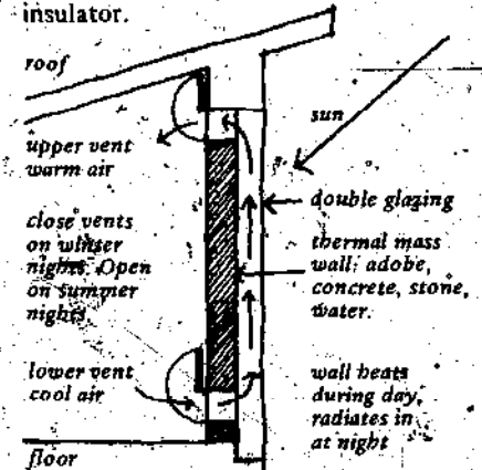
Trombe Wall — cross section from Homegrown Sundwellings
