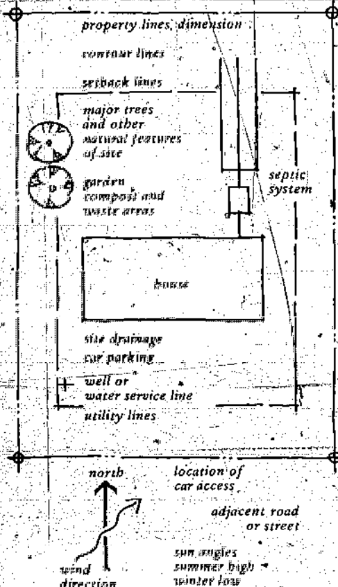
Site Plan scale
