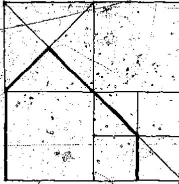
Classic New England saltbox profile, ca. 1690. After drawing by Eric Steane.
