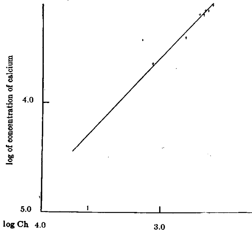
FIG. 49. Influence of B. lactis acidii upon the solubility of orthoclase (from Wright).
