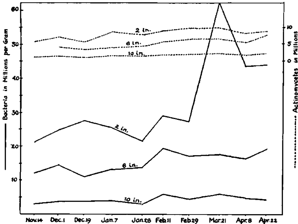
FIG. 3. Variation of numbers of bacteria and actinomyces at different seasons of the year and different depths of soil (from Lochhead).
