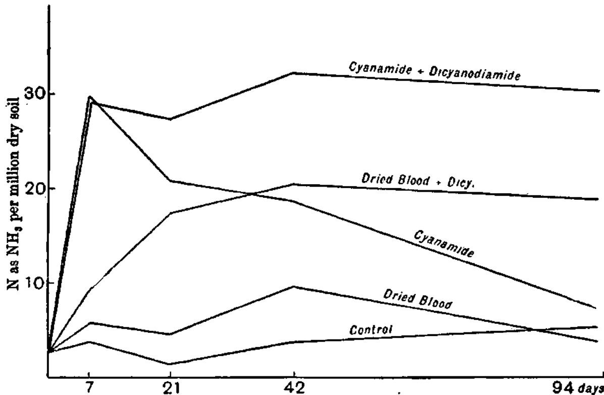
FIG. 26. Accumulation of ammonia from cyanamide and dried blood, as influenced by the presence of dicyanodiamide (from Cowie).
