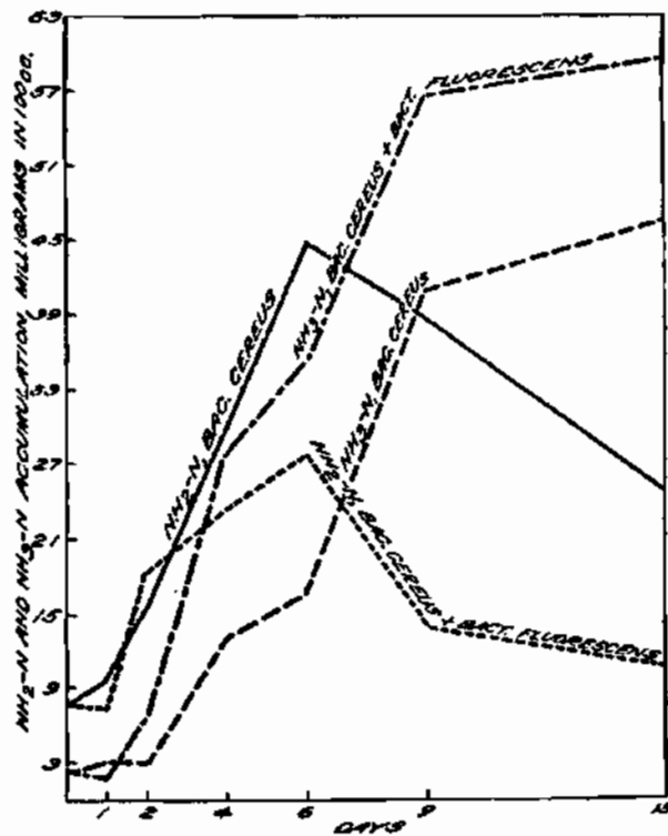
FIG. 27. Course of accumulation of amino- and ammonia-nitrogen from casein by Bac. cereus and Bact. fluorescens (from Waksman and Lomanitz).
