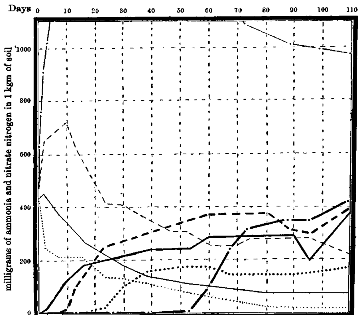
FIG. 38. Influence of organic matter upon the formation of nitrate in the soil: a, soil receiving 0.2 per cent ammonium sulfate, — nitrate N, — ammonia N; b, soil receiving 0.25 per cent peptone, — nitrate N, — ammonia N; c, soil receiving 1 per cent peptone, — nitrate nitrogen, — ammonia N; d, soil receiving 1 per cent dextrose ••• nitrate N, ..... ammonia N (after Barthel and de Rossi).
