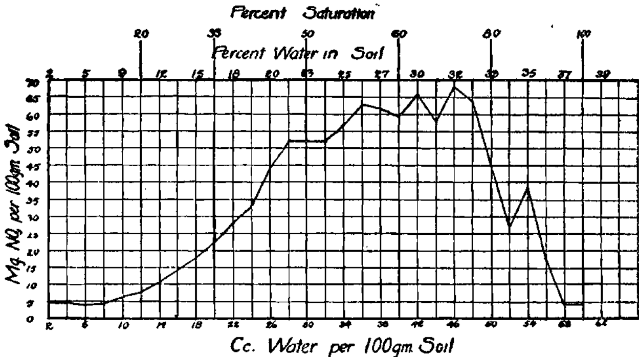
FIG. 36. Influence of moisture content upon nitrate production in the soil (from Gainey).
