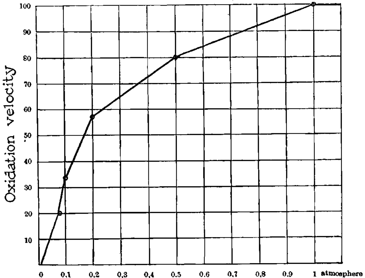
FIG. 20. Influence of oxygen pressure upon the oxidation of nitrite to nitrate (from Meyerhof).
