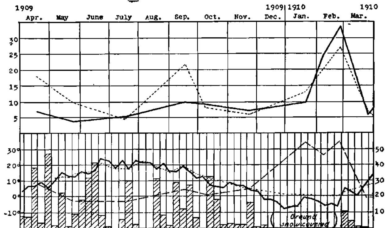
FIG. 1. Upper curves show millions of bacteria per gram of dry soil, throughout the year: ——— good soil, - - - - - poor soil; lower curves show: - - - - soil moisture in per cent; ——— atmospheric temperature; - - - - - soil temperature; shaded columns represent rainfall per week, in millimeters (from Conn).
