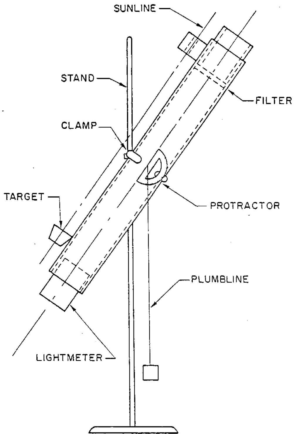
CRUDE PYRHELIOMETER
