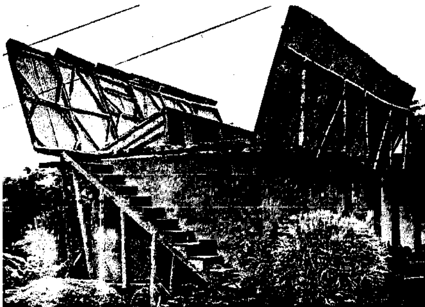
Figure 7. "Elba" house dryer The roof is put back on the house pignon for nights and rainy periods.
