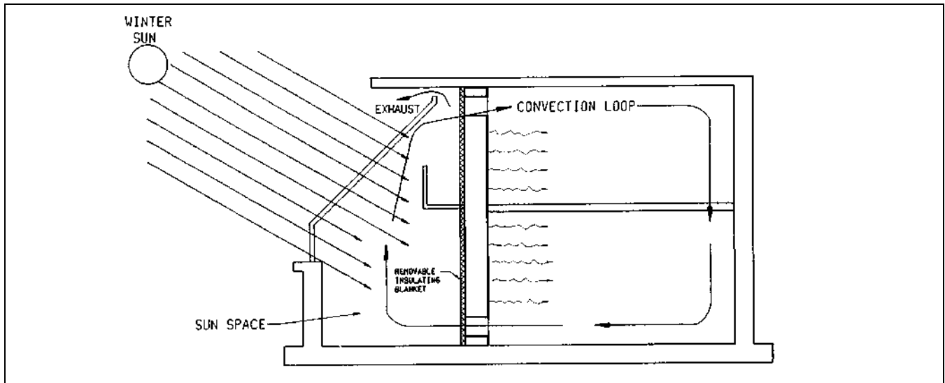
Figure 2. Isolated gain system using a sun space
