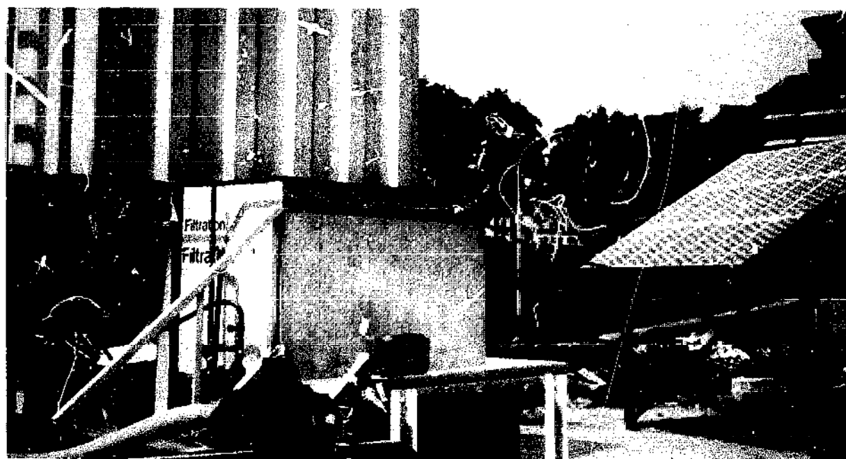
Figure 9.1 PV Water Purification Plant in Nigeria (Satec)
