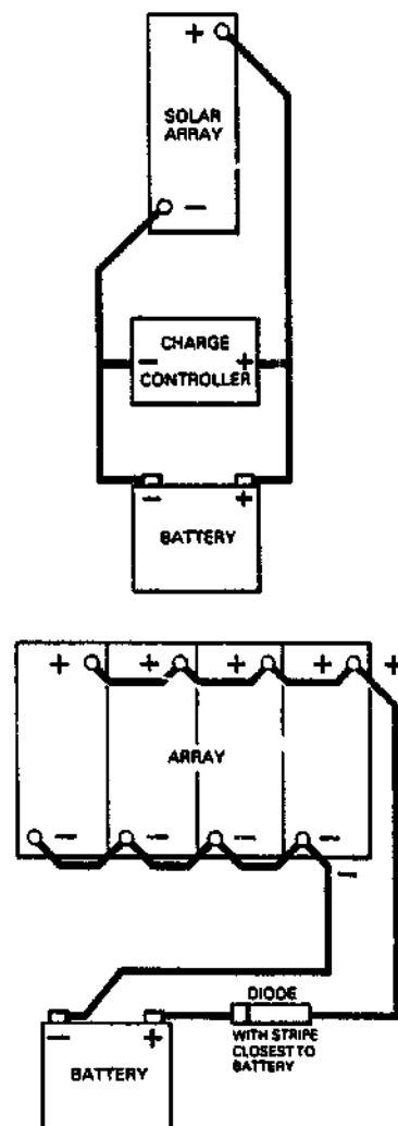
Figure 4.7 Charge Regulator and Blocking Diode Positions
