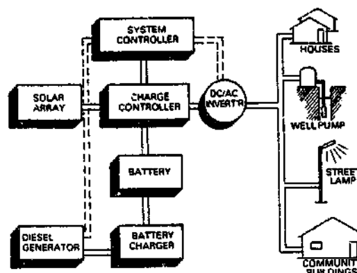
PV System with Multiple Load and Diesel Back-up
