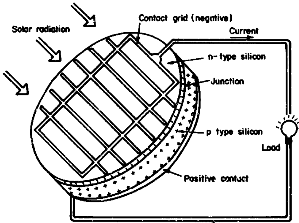
Figure 5. Construction of a silicon photovoltaic cell.
