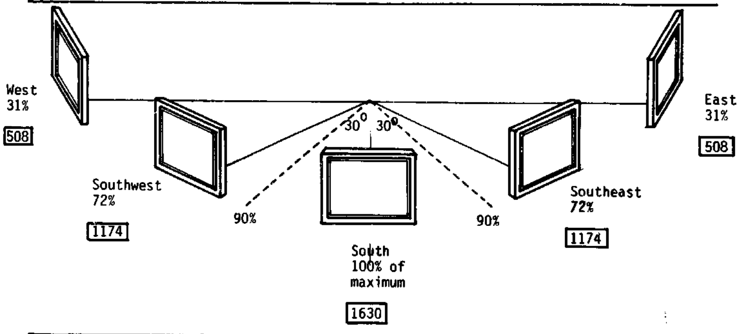
Figure 1. Solar radiation striking vertical wall relative to maximum southerly exposure (100 percent), winter condition, for the NORWESCAP latitude. Numbers in boxes represent average Btu per square foot per day solar energy striking the vertical wall in January.
