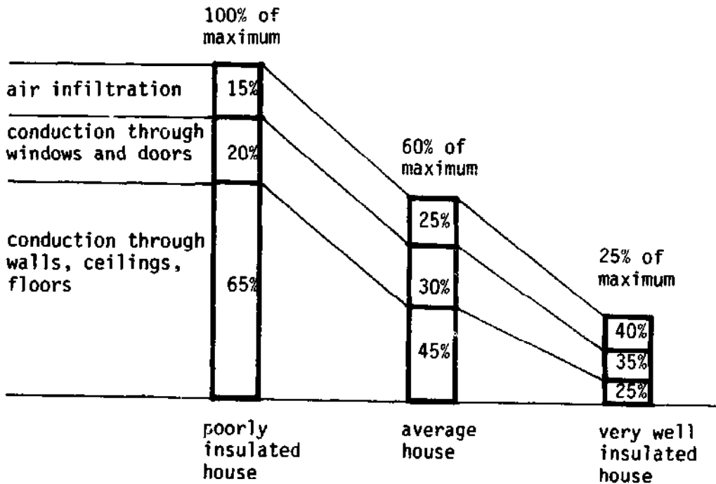
Figure 1. Comparison of heat loss due to various causes in three houses.
