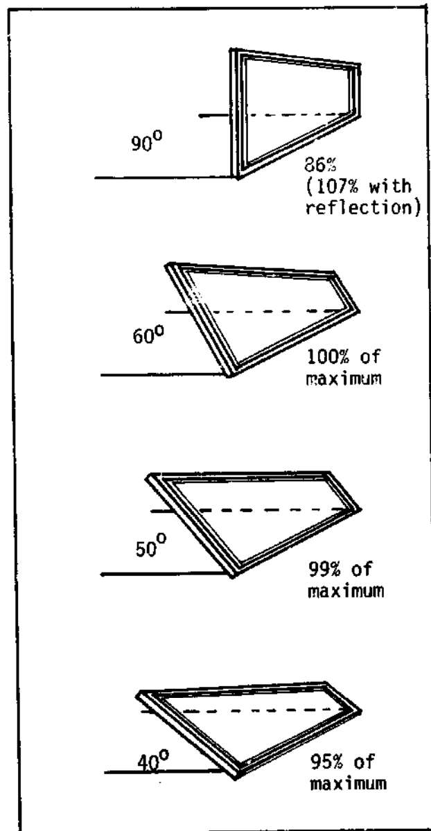
Figure 2. Solar radiation striking tilted surfaces relative to maximum (100%) 60 degree tilt angle, for the NORWESCAP latitude during the winter heating season.
