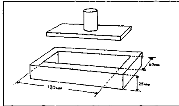
Figure 5.1: Wooden frame and ejector for making test blanks
