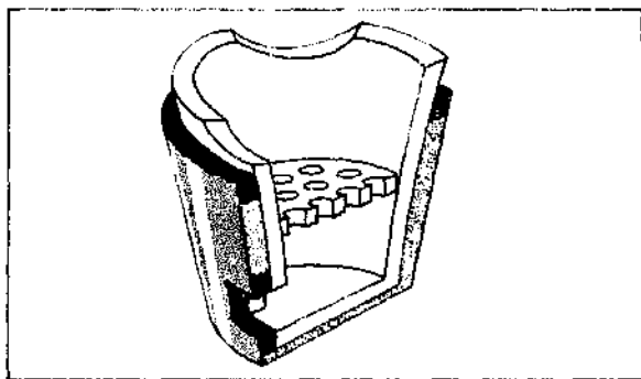
Figure 1.1: Thai Bucket stove
