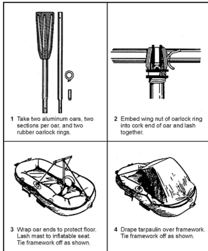
Figure 16-17. Sail Construction
