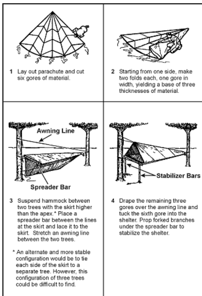
Figure 5-8. Parachute Hammock
