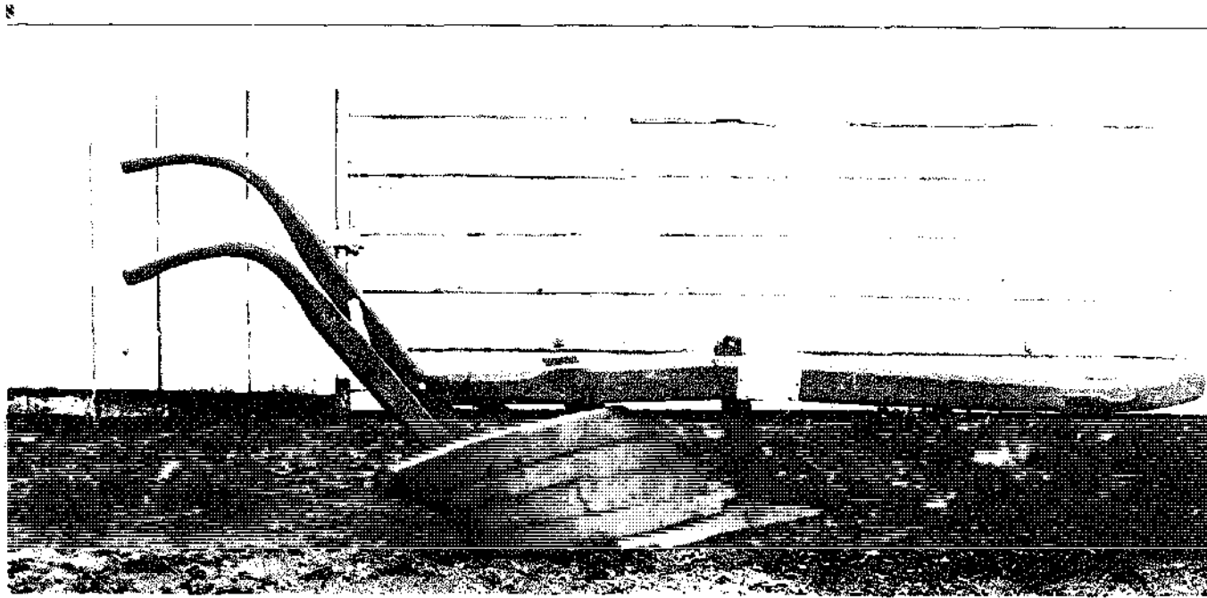
Colonial farmers in New England used the Old Colony Strong Plow to break virgin soil. The wooden moldboard was plated with thin iron strips to reduce friction and to prevent the soil from sticking to the moldboard. The iron bar in front of the moldboard is called a coulter. The coulter cuts the furrow slice vertically while the moldboard turns it over horizontally. Eastern farmers continued to use the Old Colony Plow until about 1820. It had a 10-foot beam and a 4-foot landside (the side of the plow which rested against the soil when the moldboard turned the furrow). This plow reportedly made furrows stand up like the "ribs of a lean horse in the month of March." (Smithsonian Institution.)
