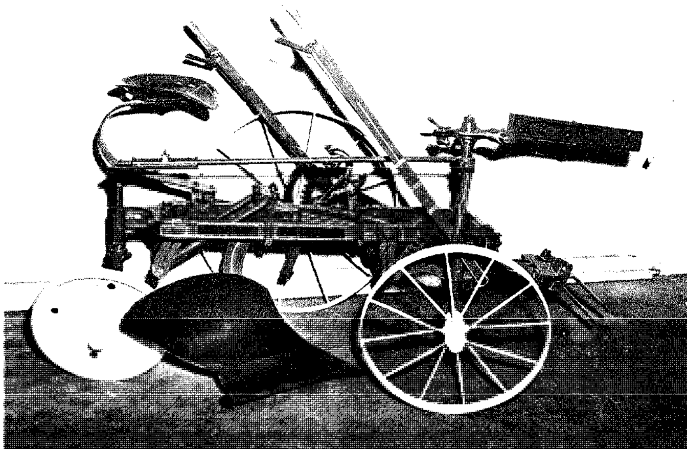
The salky or riding plow became popular in the trans-Mississippi West during the 1870s. It enabled farmers to plow faster than they could with the walking plow and to ride at the same time. The salky plow was an important tillage implement for farmers who had large acreages to prepare for seed. (Smithsonian Institution.)
