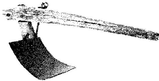
In 1837 John Deere built a plow with a highly polished wrought-iron moldboard and a steel share. It easily cut through the prairie sod and turned a furrow. John Deere made this plow in 1838, and it is probably identical to the 1837 model. He did not make a steel moldboard until 1846. The drawing shows the entire John Deere plow. (Smithsonian Institution.)
