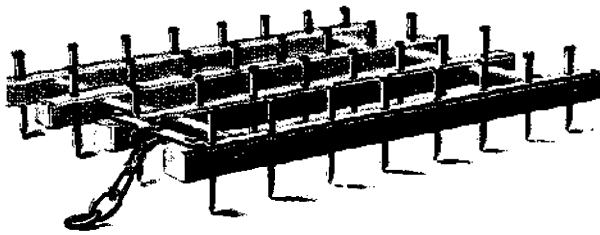
Single Section, "32 Teeth," One Horse.
