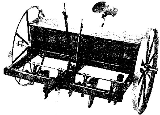
This grain drill patent model has furrow openers called "hoes." The seed fell from the grain box through tubes into the hoers. The levers enabled the farmer to set the planting depth and position of the hoers. (Smithsonian Institution.)
