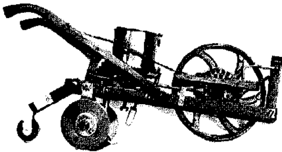
This patent model of the Hendrick's one-row corn planter (1872) shows the gearing on the front wheel which regulated the seed release mechanism under the canister. (Smithsonian Institution.)
