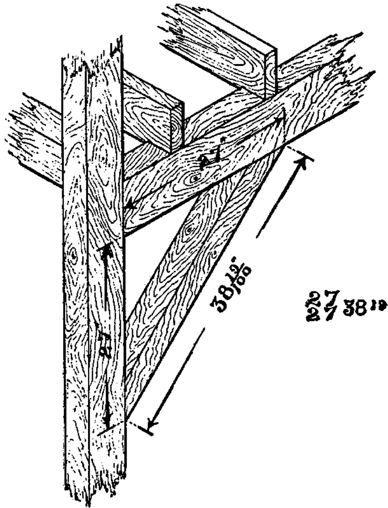
BRACE RULE
