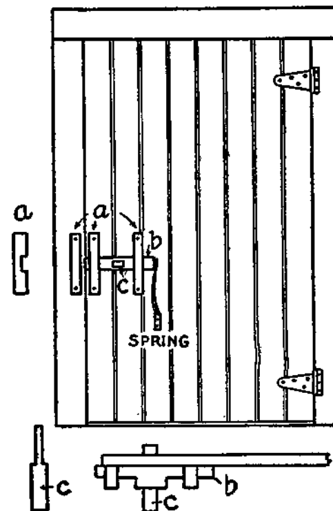
FIGURE 2—SPRING FASTENER
