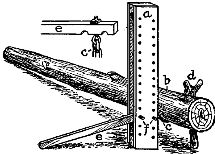
FIGURE 4—LOG JACK
