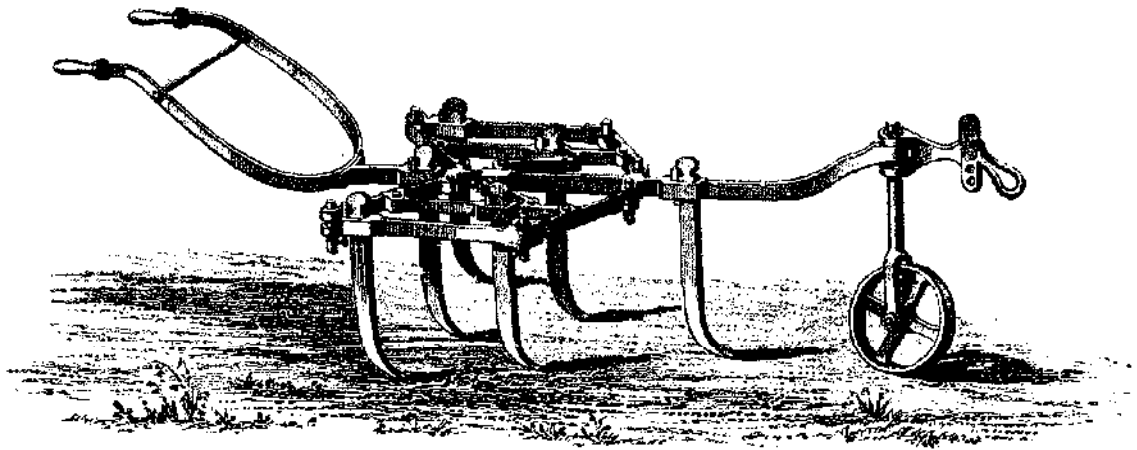
ULEY EXPANDING HOE.
