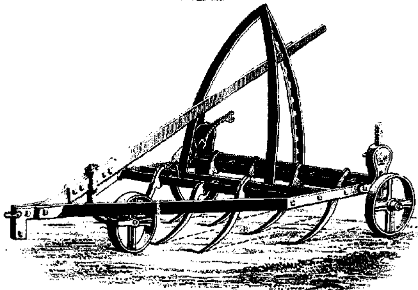
FINLAYSON'S GRUBBER. \frac{1}{4} of the full size.
