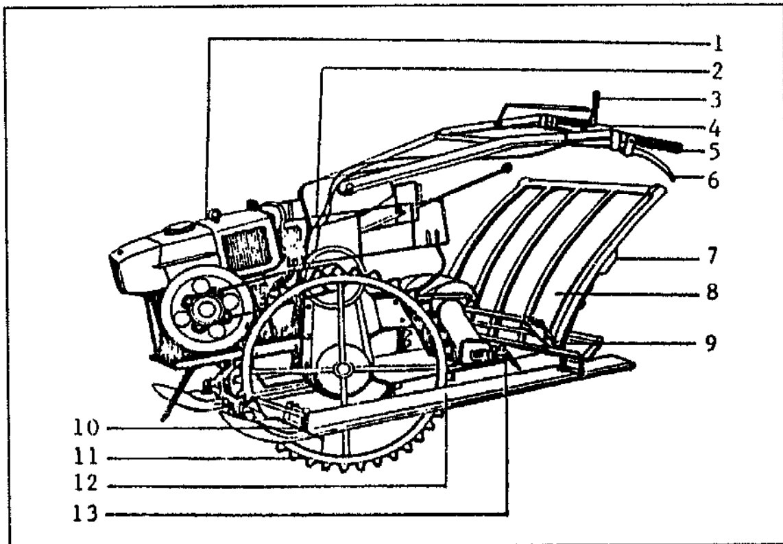
7. Schematic drawing of AMI 4-row rice transplanter using mat seedlings. 1 = engine, 2 = shelves of reserve seedlings, 3 = brake, 4 = main clutch, 5 = handle bar, 6 = side clutch, 7 = transplanter clutch, 8 = seedling tray, 9 = transplanter arm, 10 = guider, 11 = traction wheel, 12 = float, 13 = fork.
