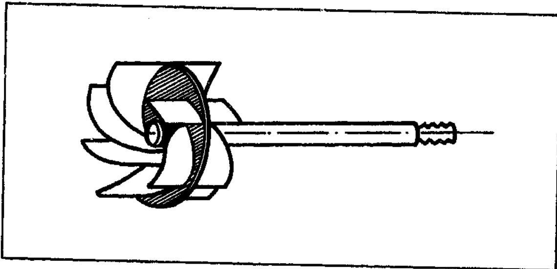
8. Double-suction impeller.
