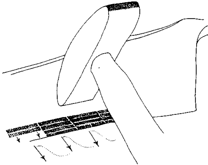
9 The sequence of hammer blows in peening.
