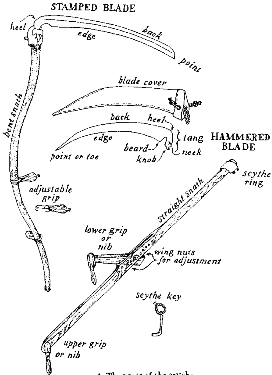
1. The parts of the scythe.
