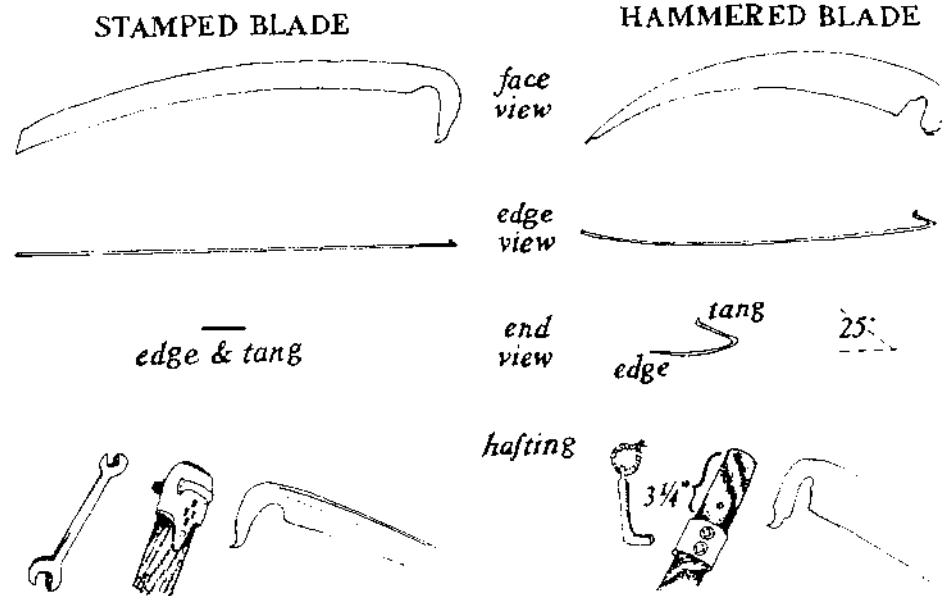
2. Stamped and hammered blades.
