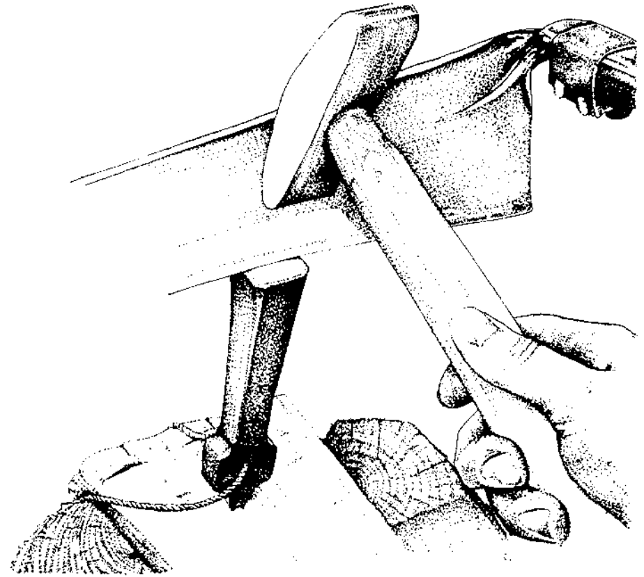
8. Peening: hammer, blade, and anvil.
