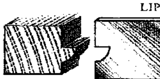
GLUE JOINT
