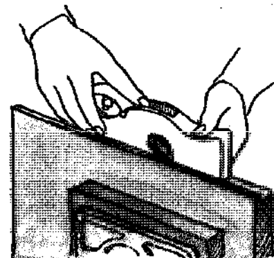
the shoulder plane two handed. Cut rabbets as with a bench rabbet plane.
