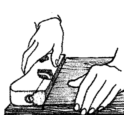
Using a shoulder plane To run on a tenon, lay a finely set shoulder plane on its side. Clamp the work in a vise to use
