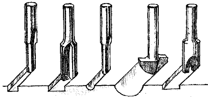
SINGLE FLUTE DOUBLE FLUTE VEINING BIT CORE BOX BIT HINGE MORTISE BIT
