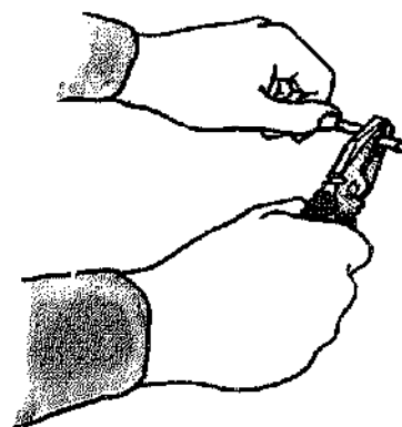
Bending a rod Hold a long rod in your hand and bend it against a pair of pliers. For shorter lengths you will need two pairs of pliers.
