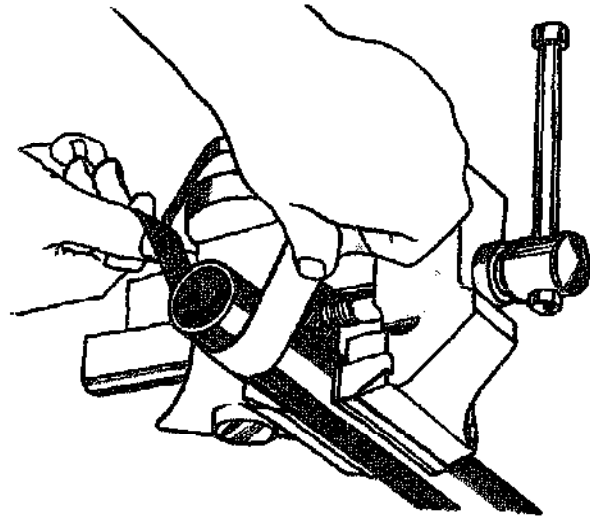
Sanding round stock Mount the work on a vise and pull cloth-backed emery strips across the surface. Angle your strokes to cover all the pipe.
