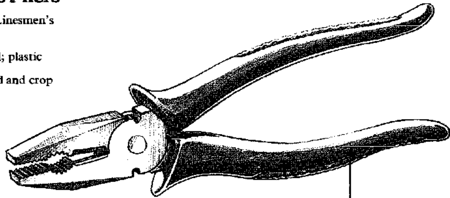
INSULATING SLEEVES
