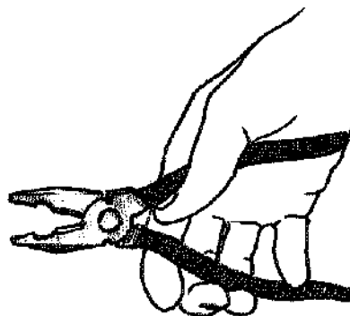
Holding the pliers To control the pliers with one hand, hook the little finger on the inside of the handle to provide the opening force.
