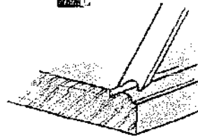
Bead with a shoulder
