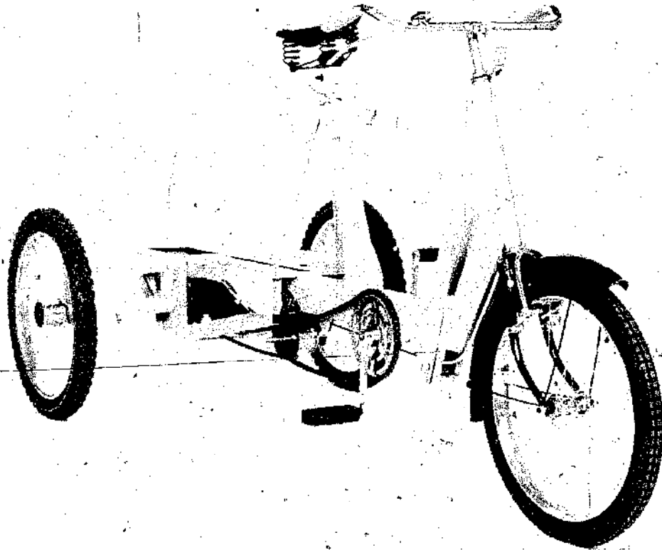
FIG 4 OXTRIKE CHASSIS
