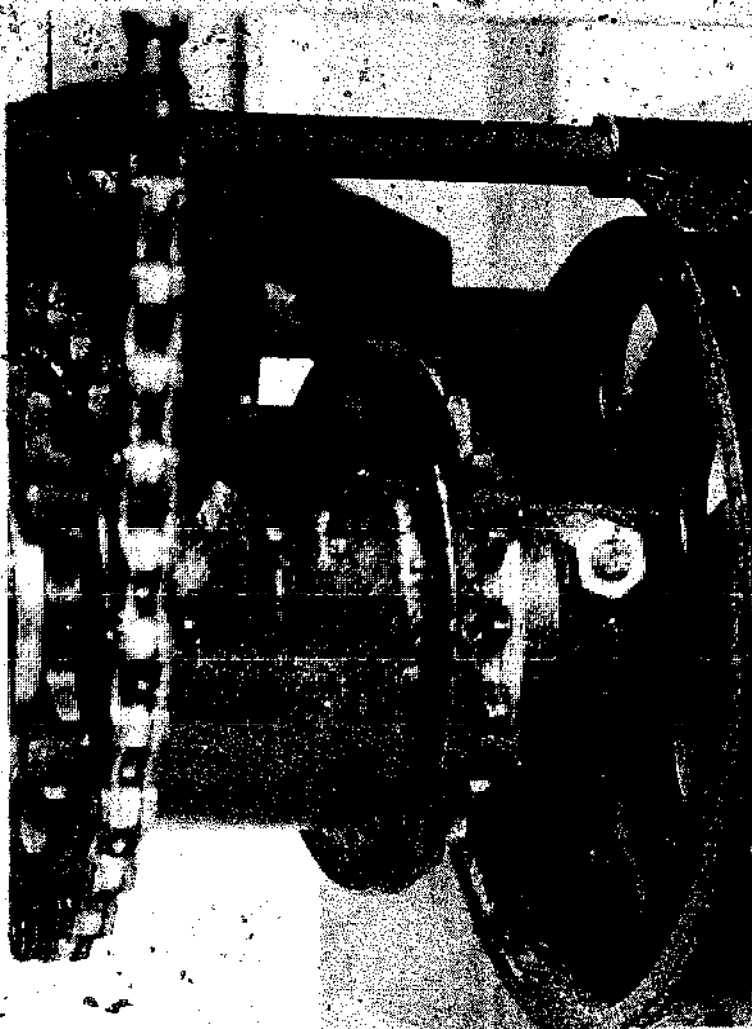
FIG 5 REAR AXLE UNIT WITH 2 FREEWHEELS, CONNECTING TUBE AND BAND BRAKES
