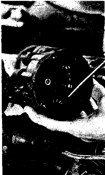
(left) To adjust the point gap, the rubbing block must be on a high lobe of the distributor cam. Some tuneup kits include a special ring that fits over the cam to hold the points open for gapping. (right) With the points held open by the cam, the gap can be adjusted to drag slightly on the specified feeler gauge. The adjustment slot is to the right of the feeler gauge and almost hidden by the wire from the condenser.
