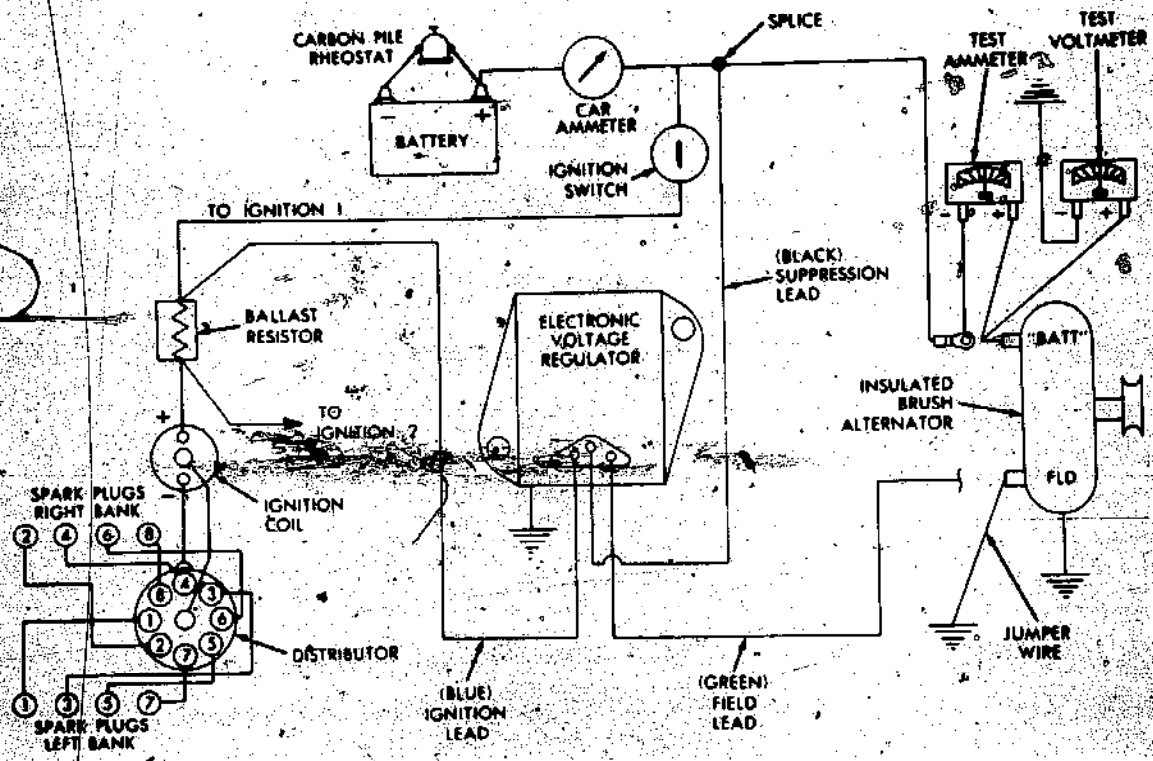
Schematic for current output test as mentioned in text.
