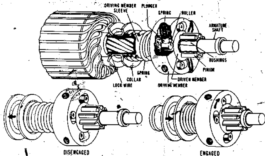
Overrunning clutch drive is used in place of Bendix drive in FoMoCo-type late model starters.
