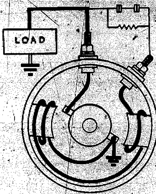
Generator with internally grounded field. Grounded brush has both its own lead and the field lead connected to it.
