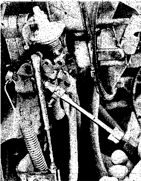
Hot idle speed is set at the solenoid or on the throttle linkage. Be sure to follow all the specifications and special procedures when setting the idle.
