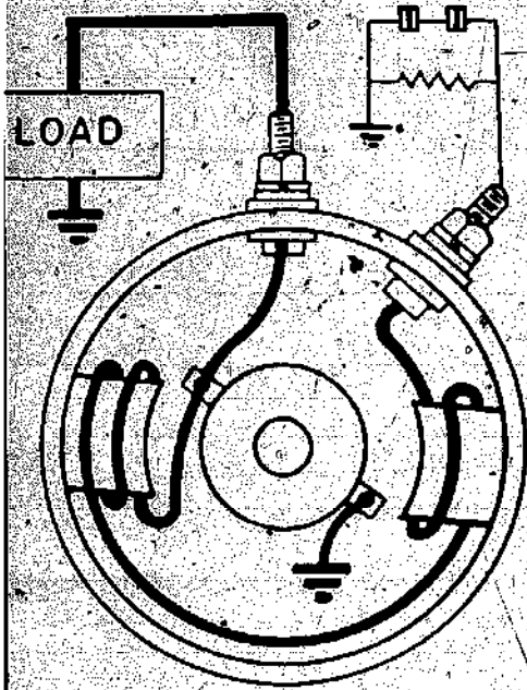
Wiring diagram of a generator having the field grounded externally through the voltage regulator. Easily identifiable because the grounded brush has only its own lead attached to it.
