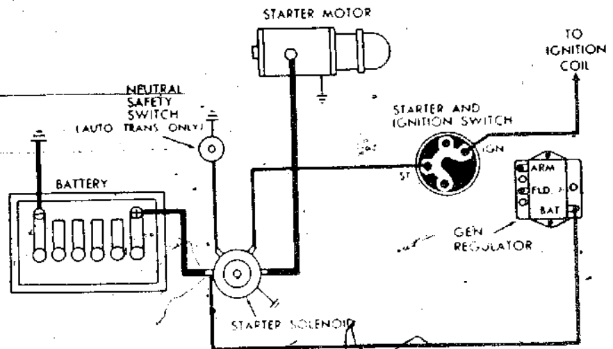
Typical starting circuit diagram shows which wires to check when shorting or bad connections are suspected.
