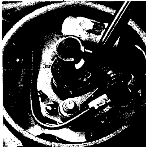
(left) To adjust the point gap, the rubbing block must be on a high lobe of the distributor cam. Some tuneup kits include a special ring that fits over the cam to hold the points open for gapping. (right) With the points held open by the cam, the gap can be adjusted to drag slightly on the specified feeler gauge. The adjustment slot is to the right of the feeler gauge and almost hidden by the wire from the condenser.
