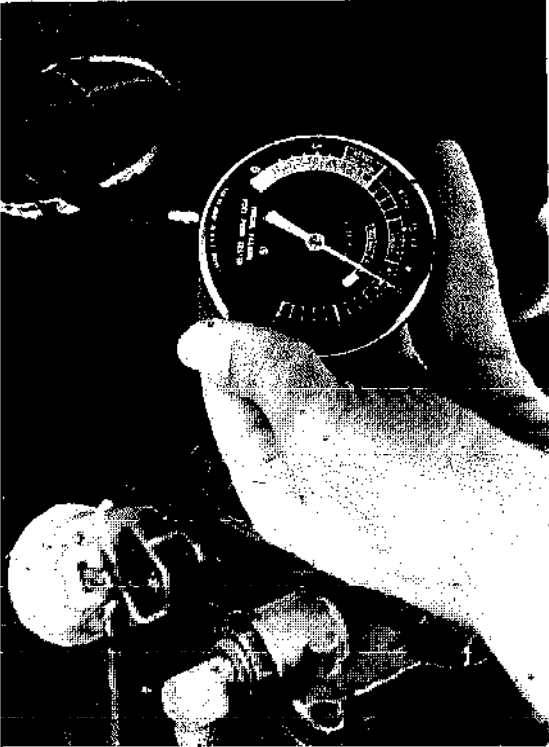
Vacuum is a good measure of an engine's performance. A steady vacuum gauge reading at idle is one of the signs of a healthy engine that can be successfully tuned.
