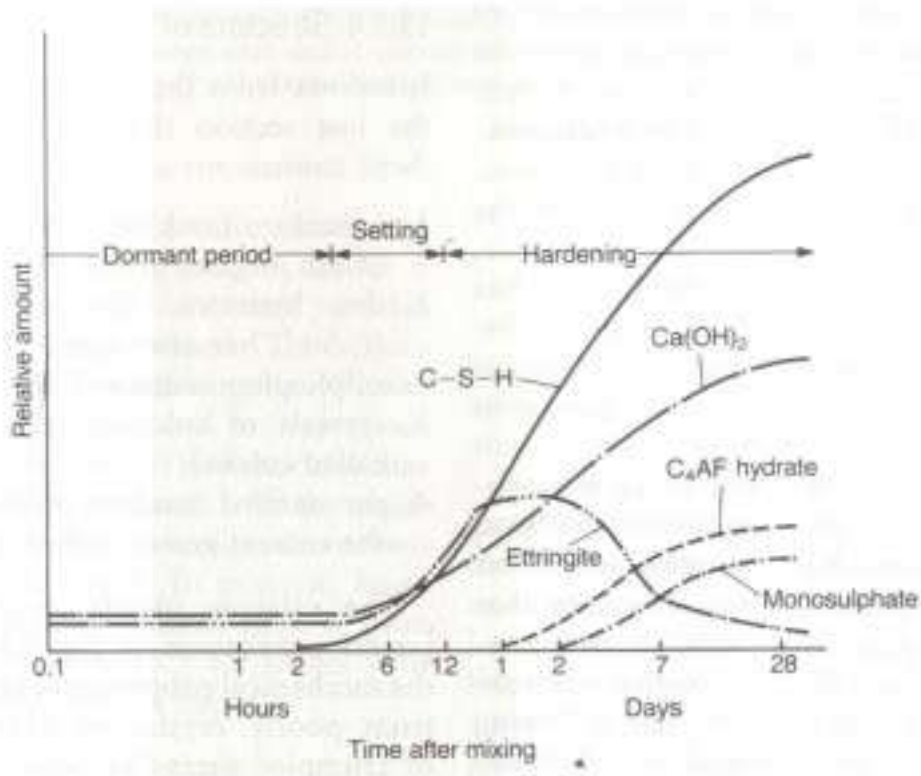
Figure 4: Typical Hydration product development in Portland cement paste (Illston 1994)
