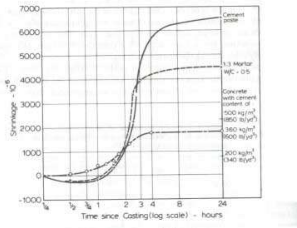
Figure A1.1.: Influence of cement content of the mix on early shrinkage (Neville 1995)
