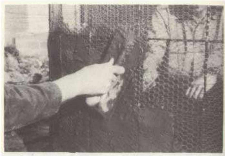
Figure 3: Construction of ferrocement tank wall (from Watt 1978)
