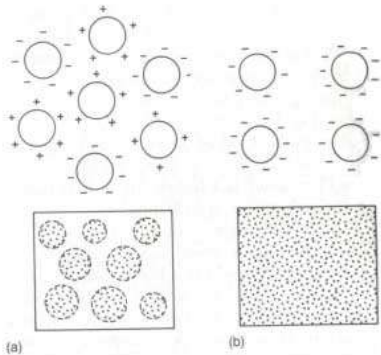
Figure 10: Dispersing action of plasticising admixtures (From Illston 1994)
