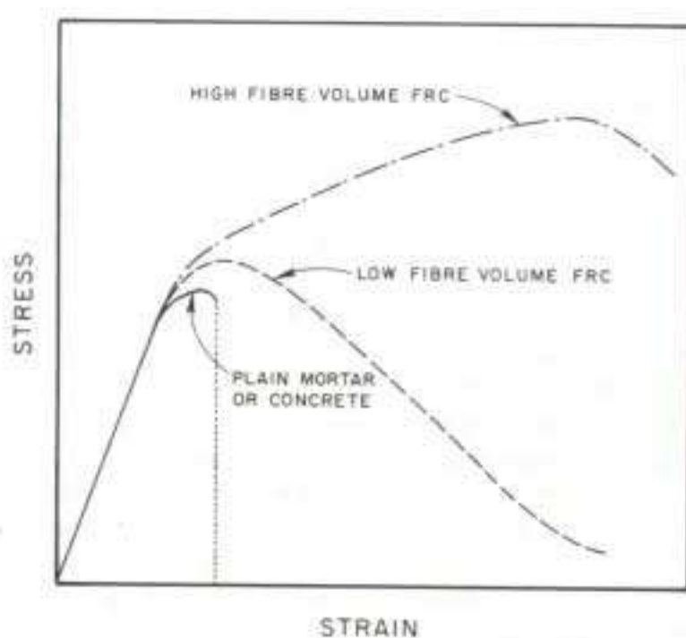
Figure 11: Typical stress-strain curves for low fibre volume and high fibre volume FRC (From Bentur 1990)
