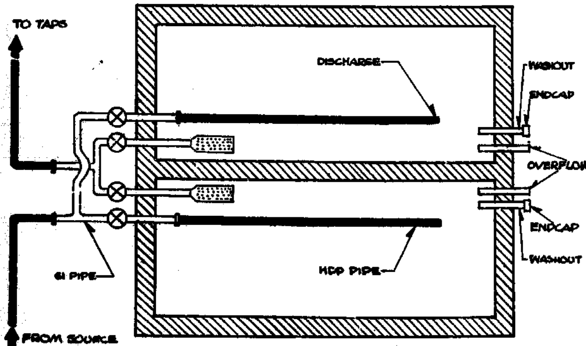
FIGURE 14-4 SERVICE PIPES FOR PARTITIONED RESERVOIR
