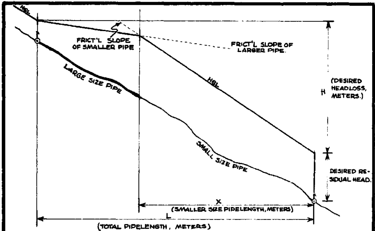
FIGURE 8-7 DESIGN EXAMPLE: COMBINATION PIPE SIZES
