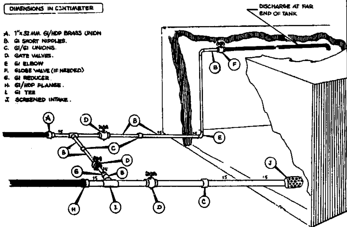
FIGURE 14-3 RESERVOIR GI PIPE ARRANGEMENT
