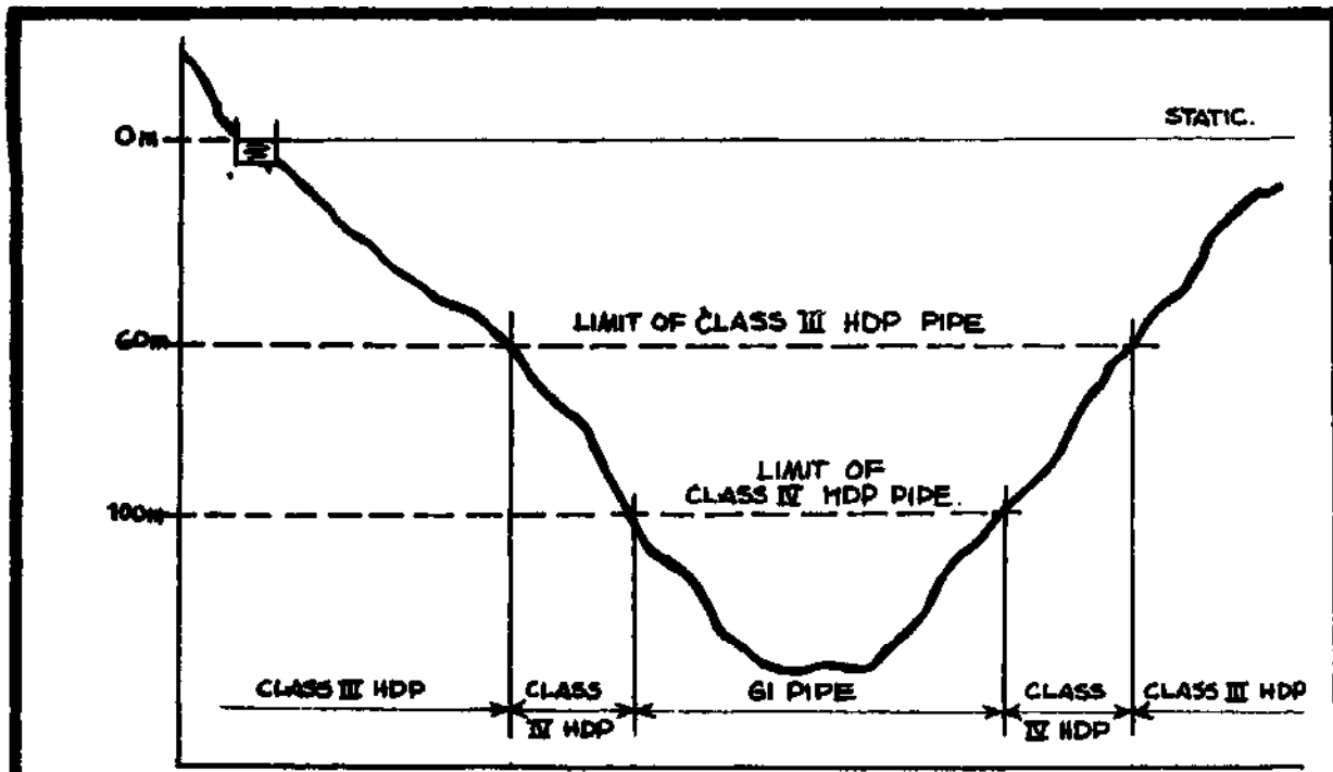
FIGURE 6-8 EXAMPLE OF U-PROFILE
