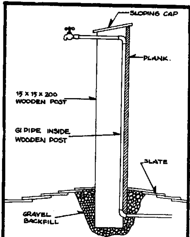
FIGURE 15-4 WOODEN TAPSTAND
