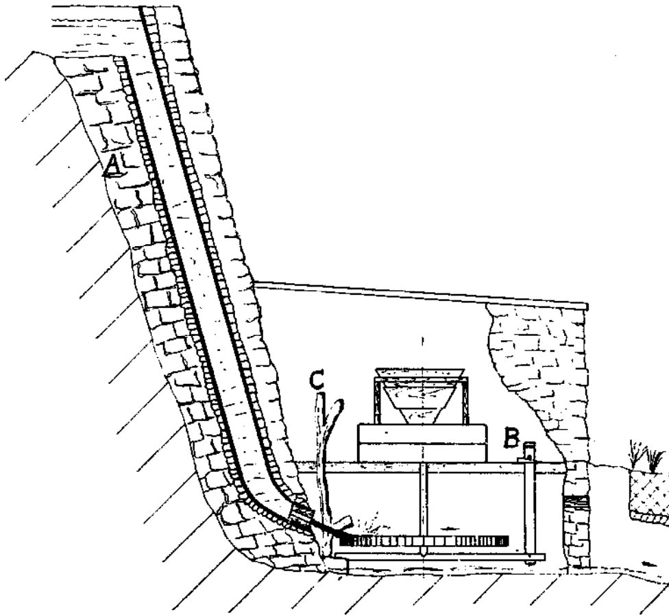
Fig. 1. Cretan water-mill.
