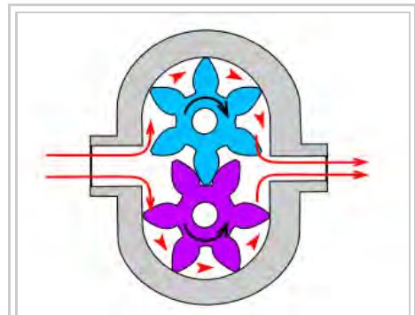
Gear pump
