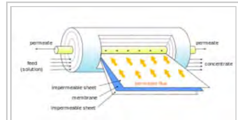
Spiral-wound membrane module
