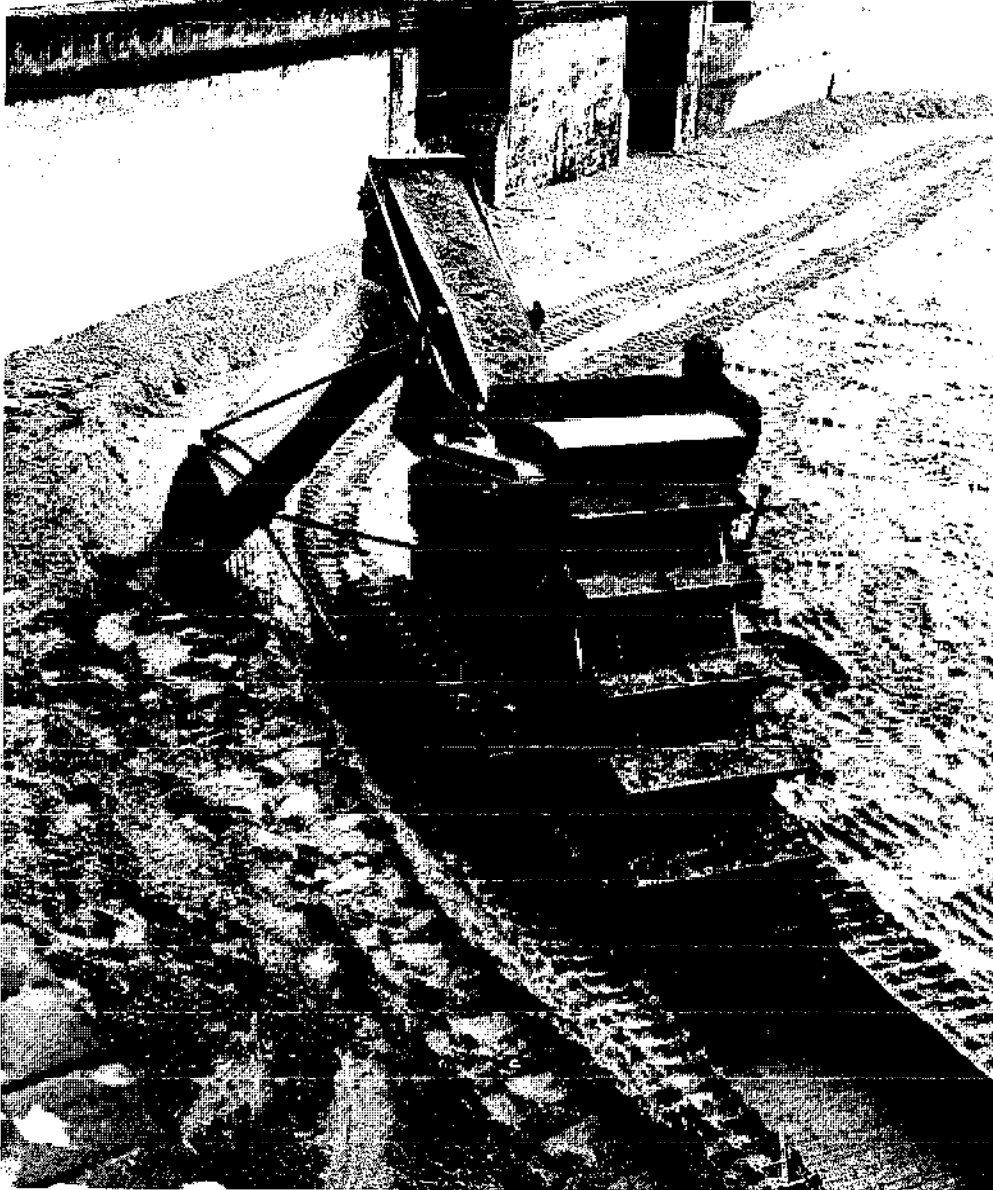
FIG. 35. TRENCHING MACHINE FOR RESANDING OPERATIONS
