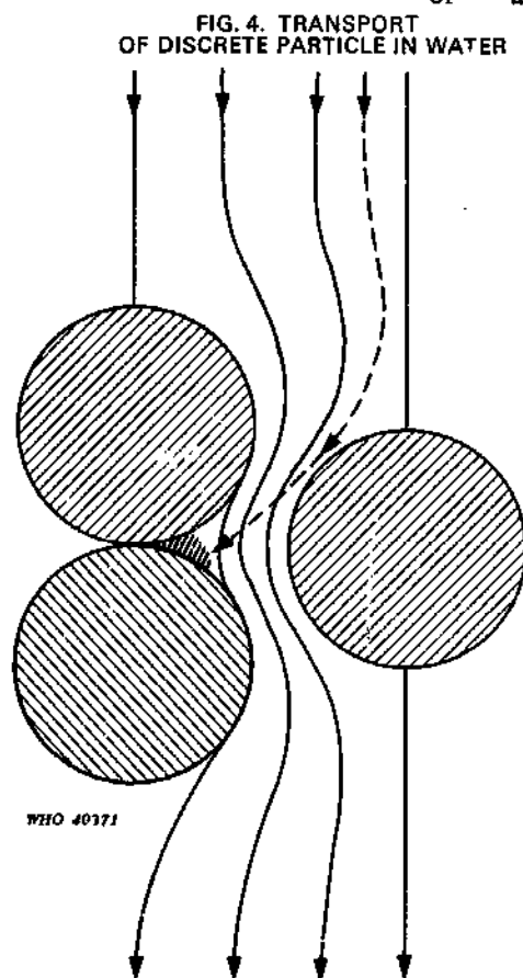
The diagram shows how inertial and centrifugal forces cause the particle to move out of the flow line and deposit in crevices between grains.
