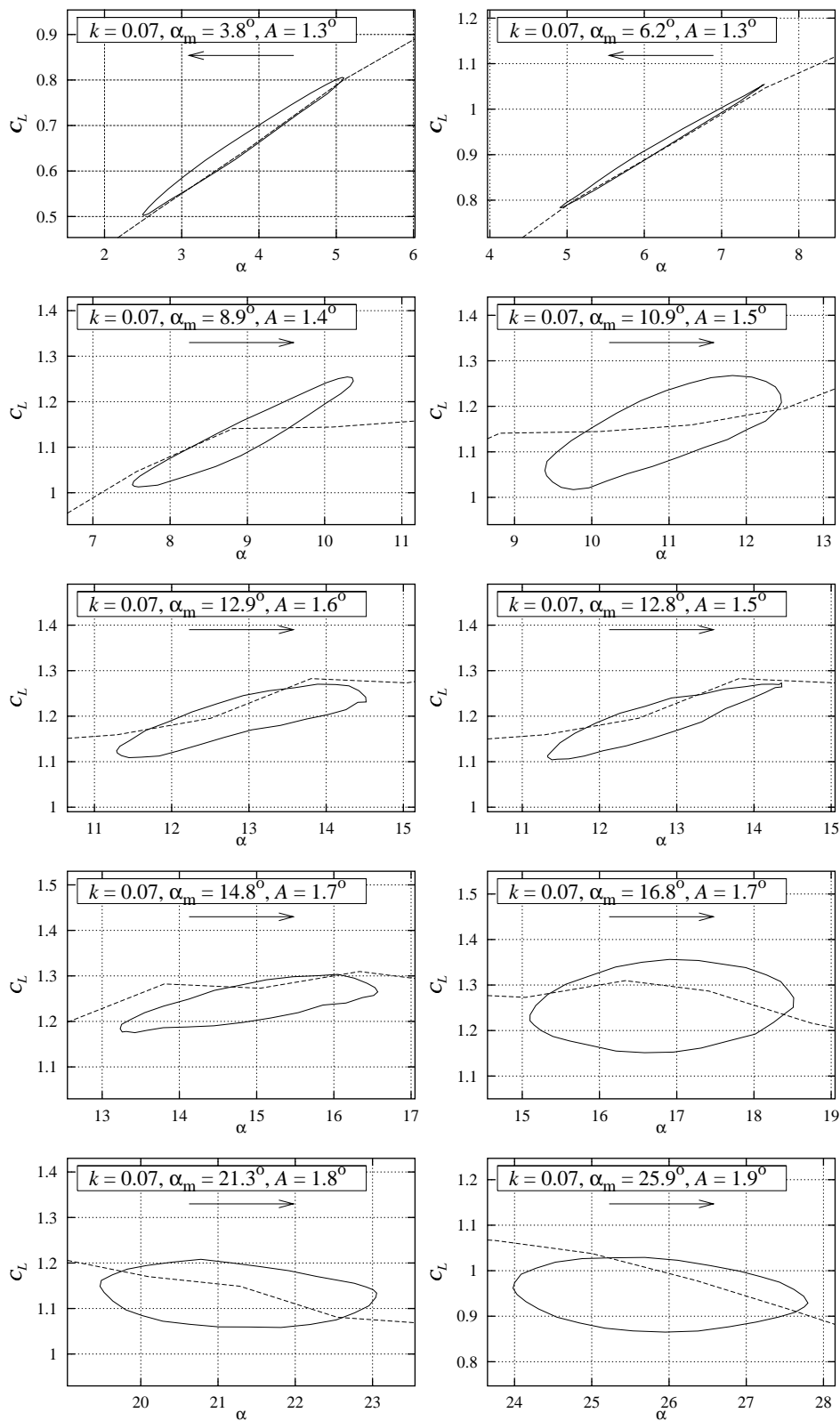
Figure G-4 Measured C_L hysteresis loops for smooth leading edge flow at k = 0.070 , A between 1.3^\circ and 1.9^\circ , Re = 1.6 \times 10^6 (FFAW3301PITCH091297V2).
