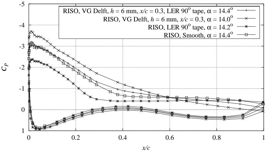
Figure D-2 Measured C_p distributions with combinations of Delft vortex generators, h = 6 \text{ mm} , x/c = 0.3 , and 90^\circ zigzag trip tape compared with smooth measurement, Re = 1.6 \times 10^6 , \alpha = 14.4^\circ (FFAW3241CONT091297V4).
