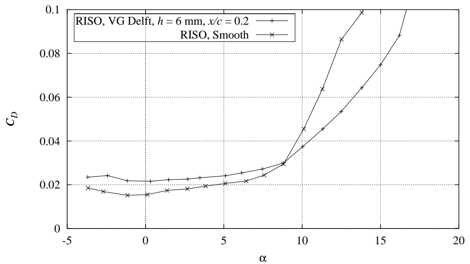
Figure F-4 Measured C_D curve with Delft vortex generators, h = 6 mm, x/c = 0.2 , compared with smooth measurement, Re = 1.6 \times 10^6 , (FFAW3301CONT091297V5).
