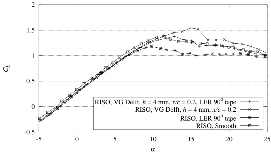
Figure D-9 Measured C_L curves with combinations of Delft vortex generators, h = 4 mm, x/c = 0.2 , and 90^\circ zigzag trip tape compared with smooth measurement, Re = 1.6 \times 10^6 (FFAW3241CONT091297V8).
