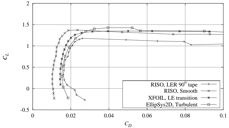
Figure C-5 Measured C_L - C_D curve for 90^\circ zigzag trip tape compared with smooth measurement and XFOIL (LE transition) and EllipSys2D (turbulent) calculations, Re = 1.6 \times 10^6 (FFAW3241CONT091297V5).
