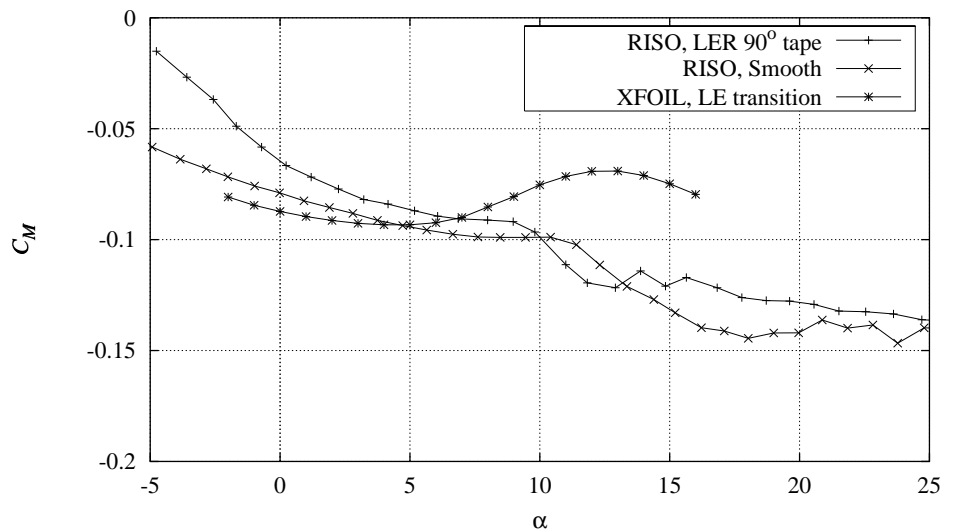
Figure C-6 Measured C_M curve for 90^\circ zigzag trip tape compared with smooth measurement and XFOIL (LE transition) calculations, Re = 1.6 \times 10^6 (FFAW3241CONT091297V5).
