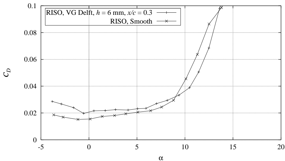
Figure F-10 Measured C_D curve with Delft vortex generators, h = 6 mm, x/c = 0.3 , compared with smooth measurement, Re = 1.6 \times 10^6 , (FFAW3301CONT091297V1).
