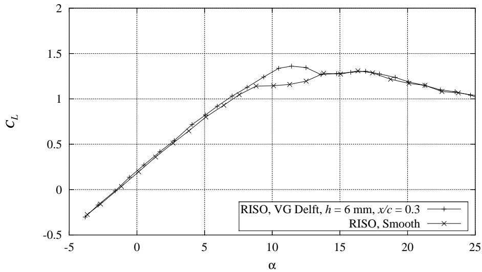
Figure F-9 Measured C_L curve with Delft vortex generators, h = 6 mm, x/c = 0.3 , compared with smooth measurement, Re = 1.6 \times 10^6 , (FFAW3301CONT091297V1).
