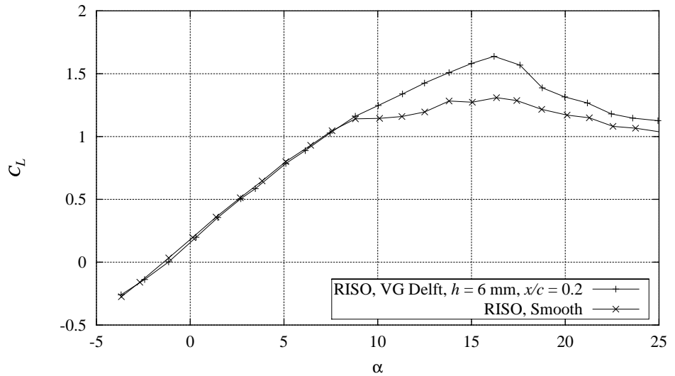
Figure F-3 Measured C_L curve with Delft vortex generators, h = 6 mm, x/c = 0.2 , compared with smooth measurement, Re = 1.6 \times 10^6 , (FFAW3301CONT091297V5).
