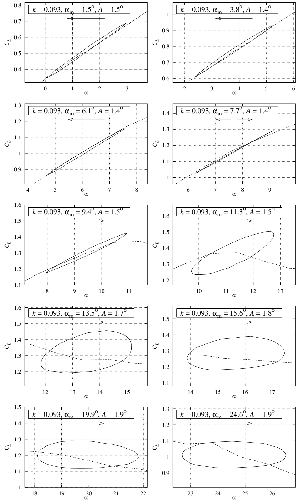
Figure E-1 Measured C_L hysteresis loops for smooth leading edge flow at k = 0.093 , A between 1.4^\circ and 2^\circ , Re = 1.6 \times 10^6 (FFAW3241PITCH091297V1).
