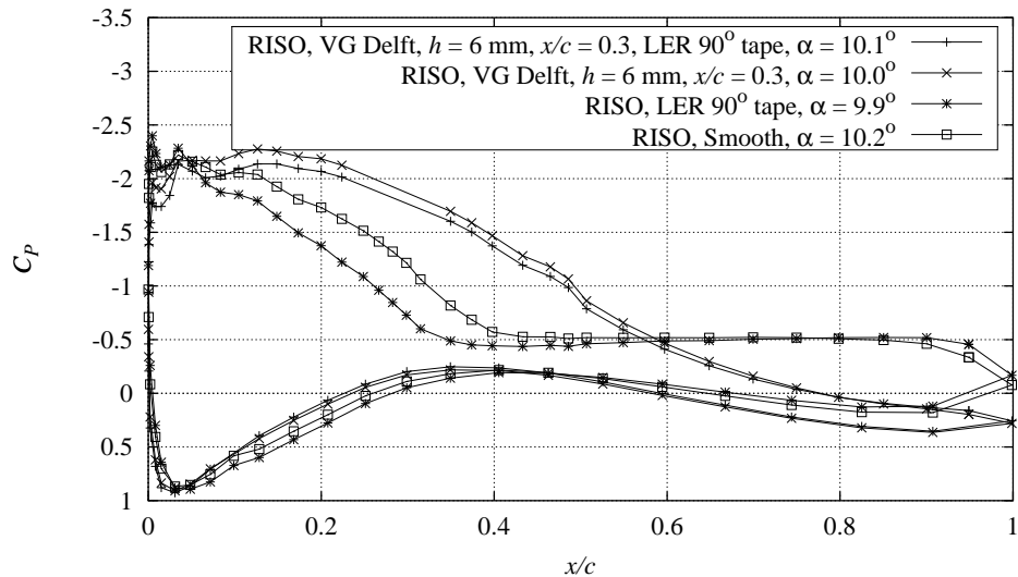
Figure 17-2 Measured C_p distributions with combinations of Delft vortex generators, h = 6 \text{ mm} , x/c = 0.3 , and 90^\circ zigzag trip tape compared with smooth measurement, Re = 1.6 \times 10^6 , \alpha = 10.1^\circ (NACA63430CONT091297V2).
