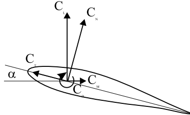
Figure 2-4 Sign convention for aerodynamic coefficients.
