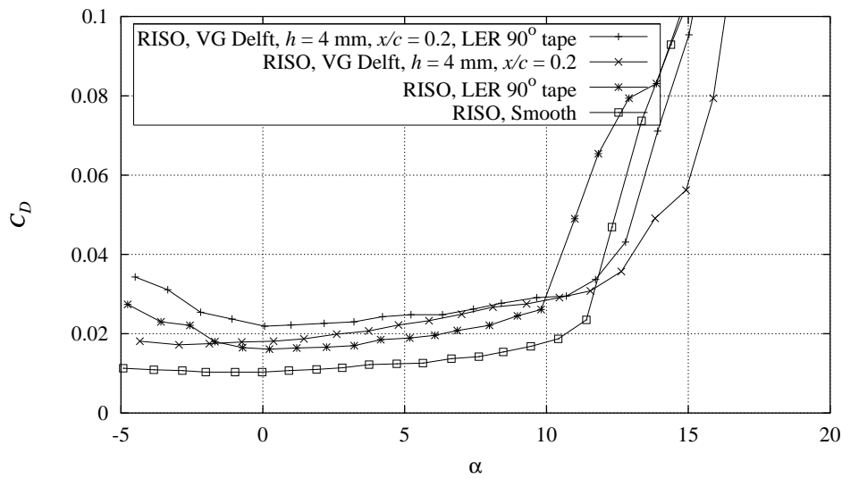
Figure D-10 Measured C_D curves with combinations of Delft vortex generators, h = 4 mm, x/c = 0.2 , and 90^\circ zigzag trip tape compared with smooth measurement, Re = 1.6 \times 10^6 (FFAW3241CONT091297V8).
