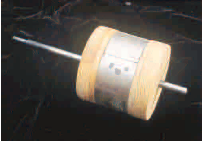
The wooden armature holds eight NdFeB (neodymium-iron-boron) magnets arranged in alternating polarity around its perimeter.
