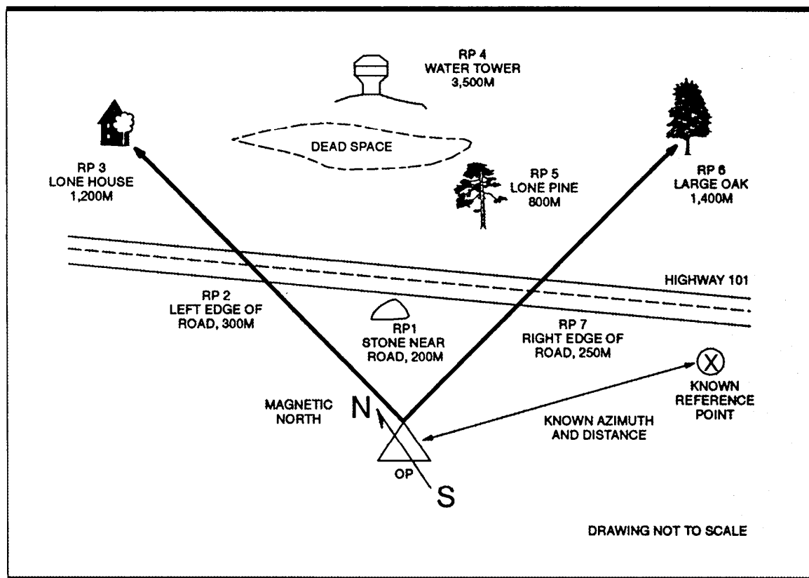
Figure C-7. Reference point diagram.
