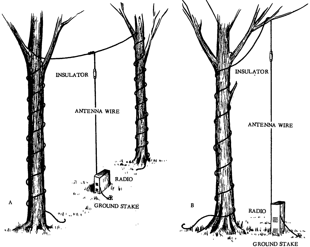
Figure 132. Vertical wire expedient antennas.
