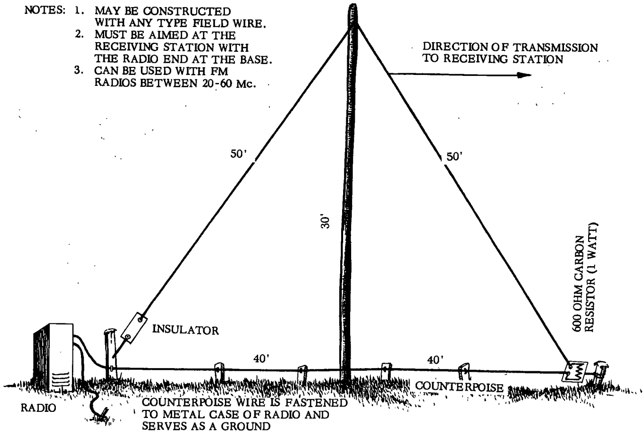
Figure 130. Half-rhombic field expedient antenna.
