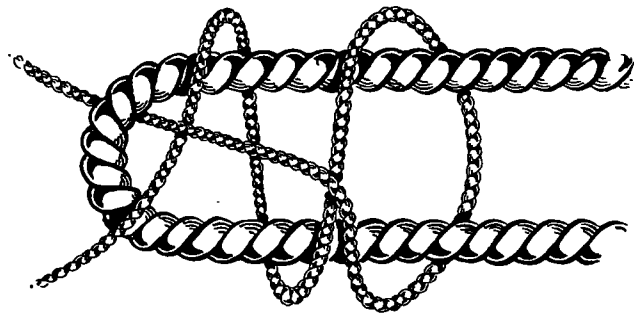
Figure 114. Sheet bend. To join wet ropes and ropes of unequal diameter.
