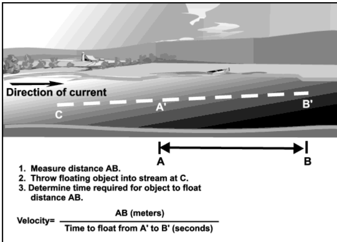
Figure 9-5. Measuring stream velocity.
