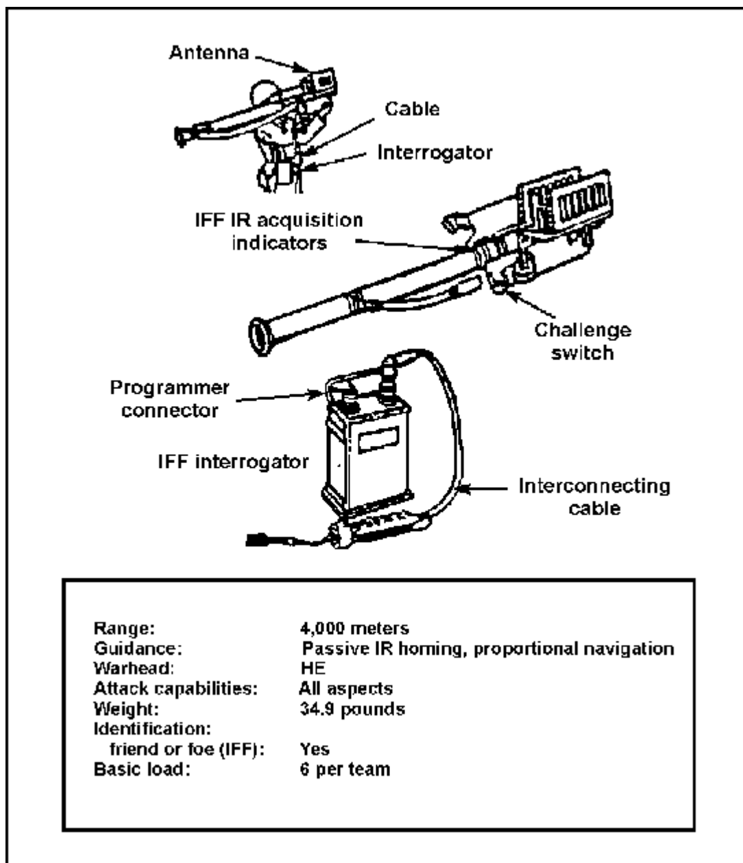
Figure 6-17. Stinger air defense system.
