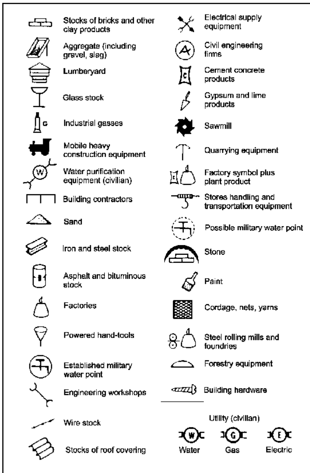
Figure 9-3. Material, facility, equipment, and service symbols.
