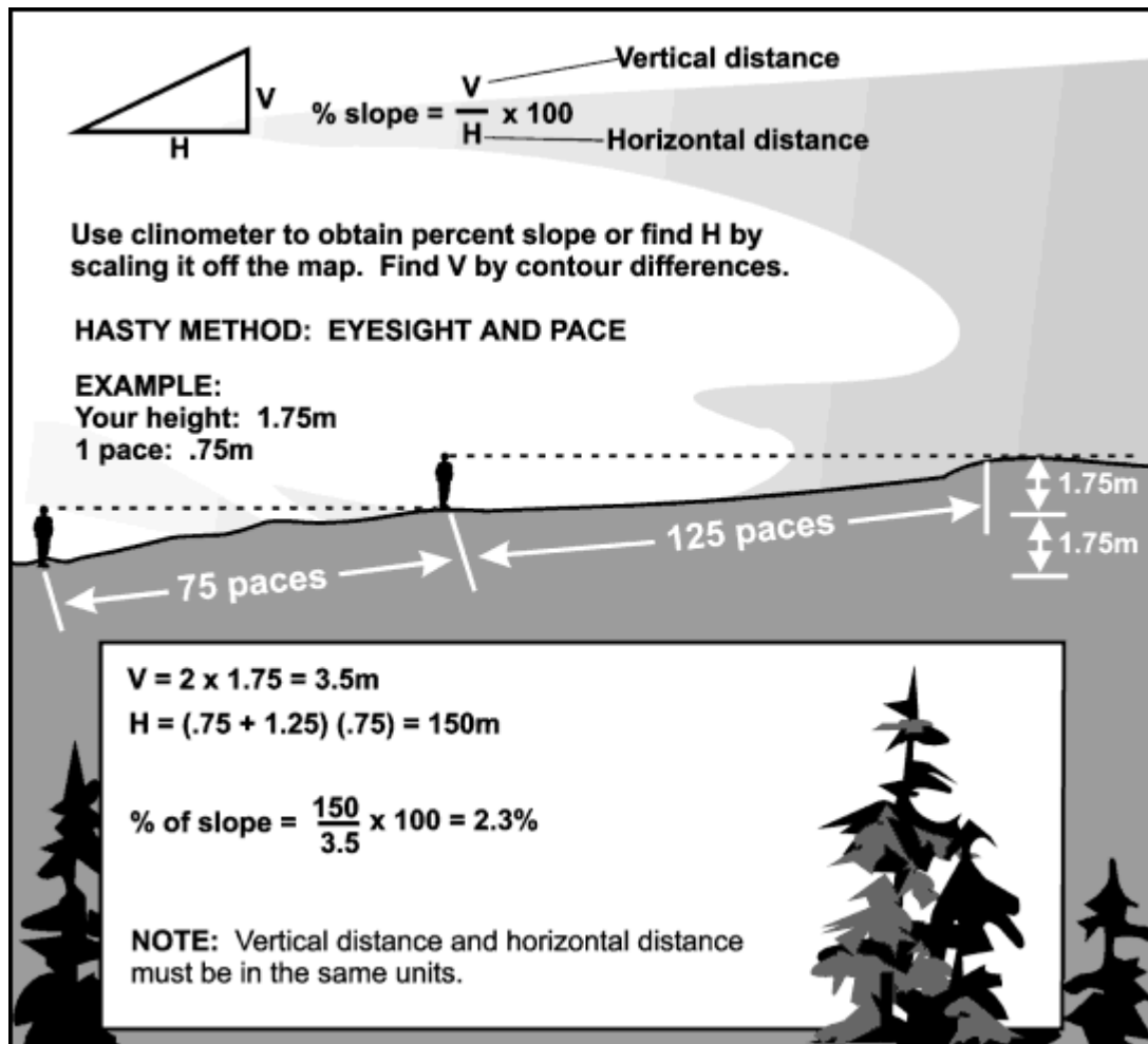
Figure 9-6. Slope computation (road gradient).
