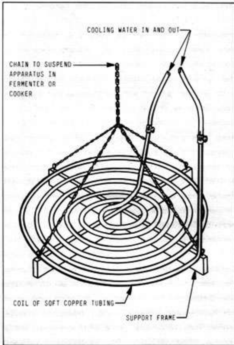
Figure 13-4: COOLING COIL
