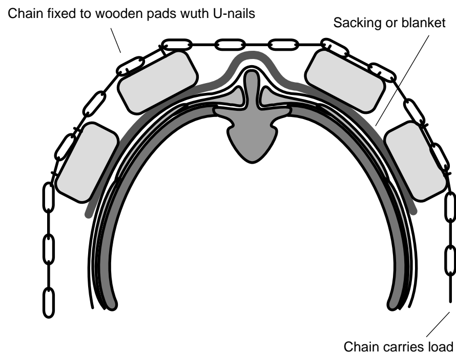
Figure 5: height of wooden blocks keeps chain away from backbone. Note sacking/ blanket padding.
