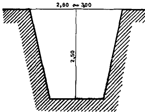
Fig. 10 Section of a silage trench
