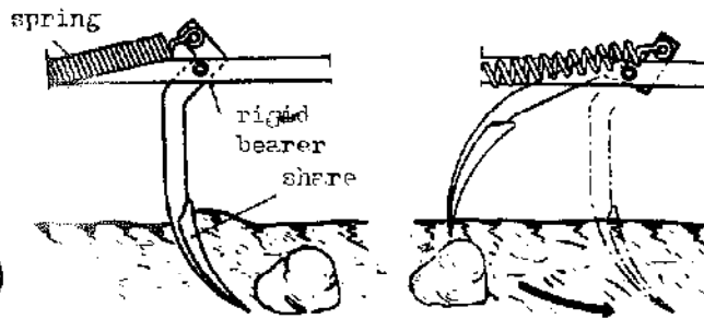
Fig. 69 - Retractable rigid tine-spring loaded
