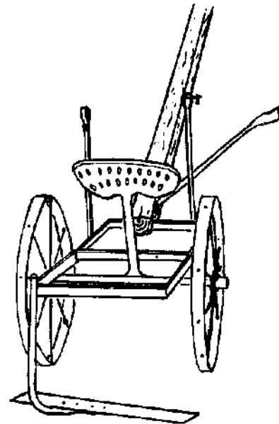
Fig. 152 -Lifter on frame with wheels
