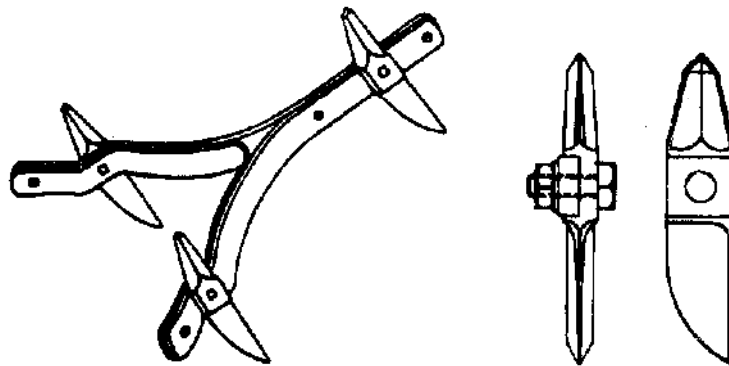
Fig. 78 - Reversible teeth for spike tooth harrows
