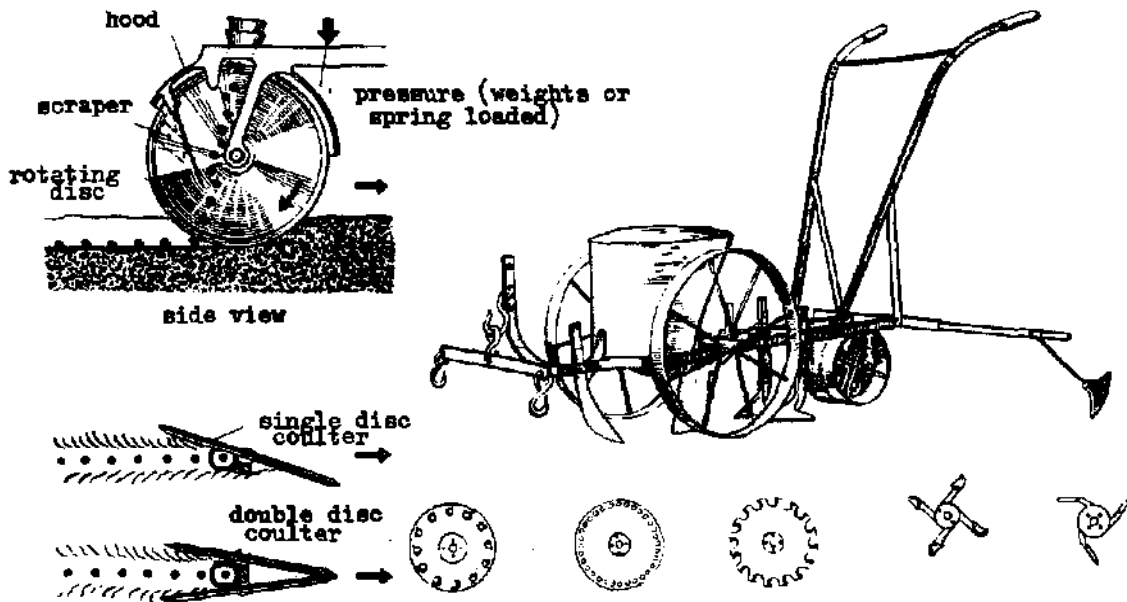
Fig. 110 - Seed planter. General view: Distribution plates and star wheels, interchangeable for different types of seeds.
