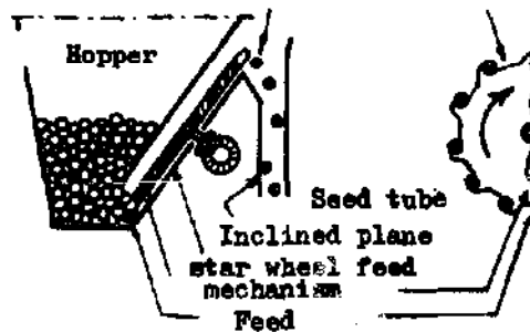
Fig. 112 - Planter with star wheel feed
