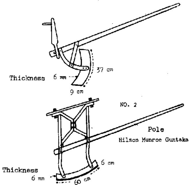
Fig. 151 - Improved "Guntakas" used in India
