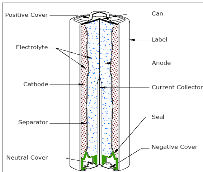
(fig. 4) Typical Cylindrical Alkaline Battery
