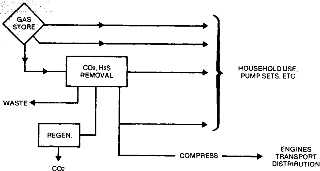
Fig. 18. Alternative treatments and end uses of the gas from the digestion process.
