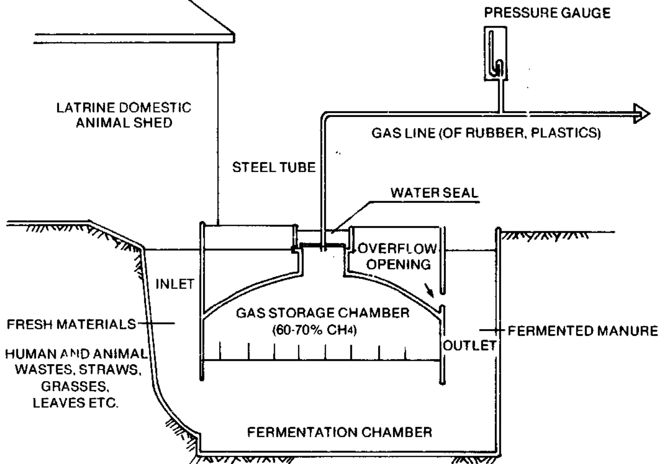
Fig. 15. This ingenious digester design of Chinese origin can handle animal manures and some vegetable wastes. It is constructed entirely of brick and cement and incorporates no moving parts.
