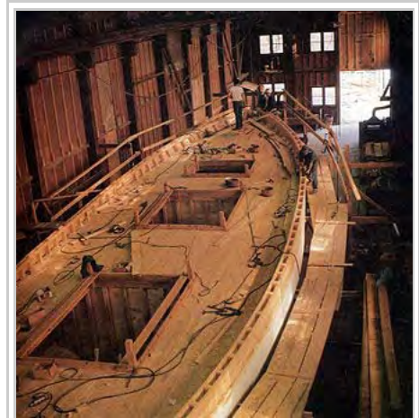
The schooner Appledore II under construction.
