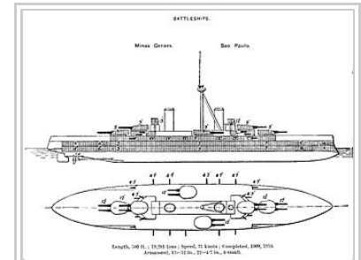
Diagram showing the Minas Geraes -class battleship with its central guns arranged en echelon .
