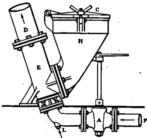
Figure 61.—Ash Ejector.
