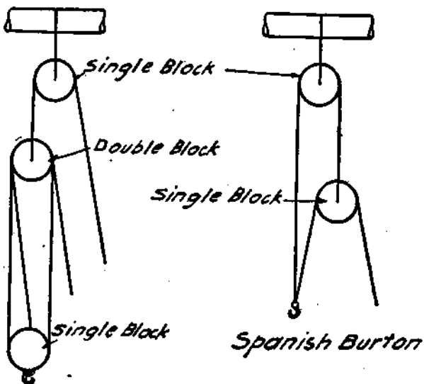
Runner's Tackle
