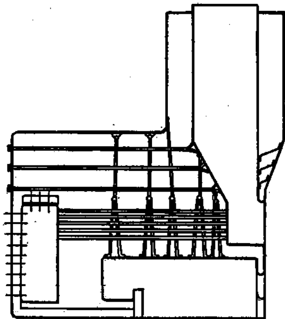
Figure 55.—Leg Boiler.
