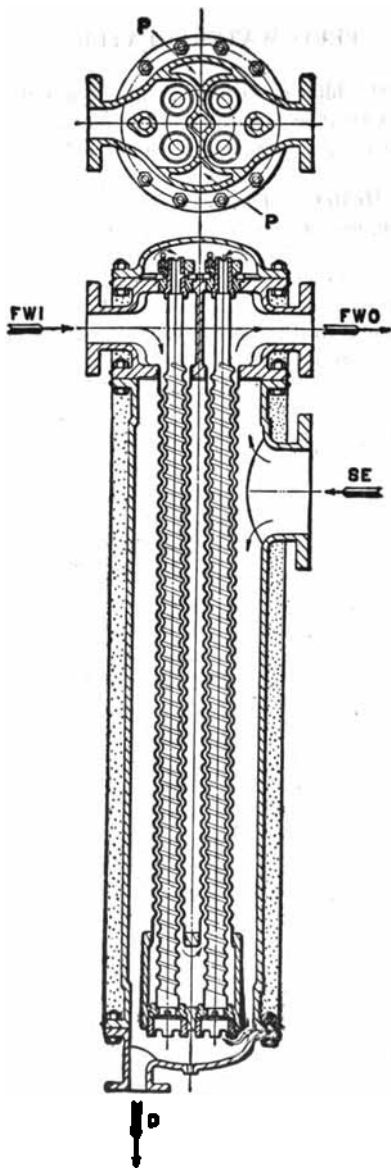
Figure 90.—Feed Water Heater.
