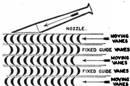
Velocity Compounding (A. E. G. (Small), Electric and Terry)
