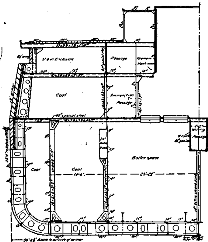
Figure 35.—Midship Section of a Battleship.
