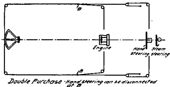
Figure 102.—Hand and Steam Steering Arrangements.
