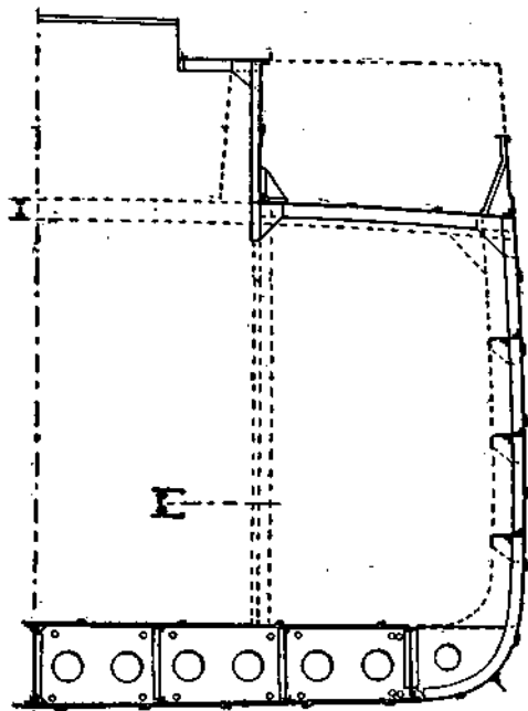
Figure 37.—Midship Section of a Trunk Vessel.
