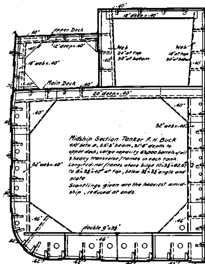
Figure 40.—Longitudinal or laborwood System.
