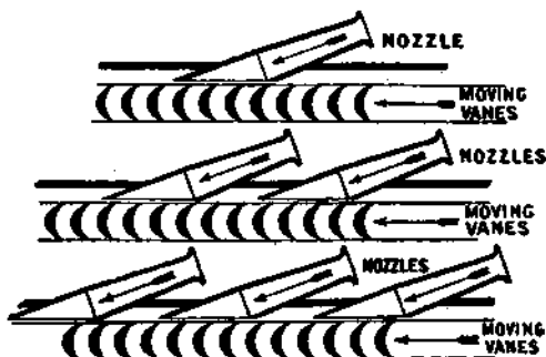
Figure 72.—Arrangement of Vanes.
