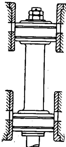
Figure 63.—Piston Valve.
