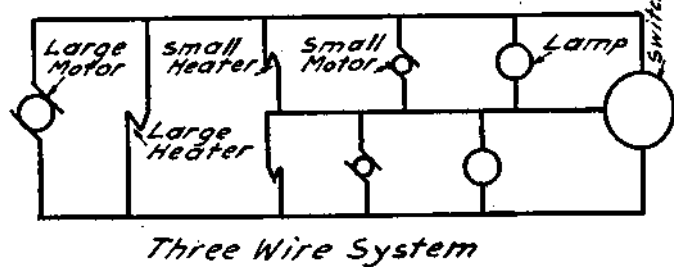
Figure 90.—Wiring Diagrams.
