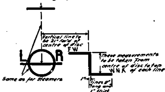
Figure 32.—Freeboard Markings
