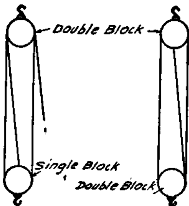
Luff Tackle
