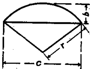
Figure 4 Spherical Sector
