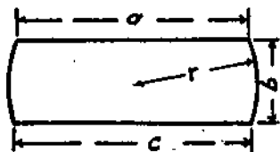
Figure 6 Spherical Zone
