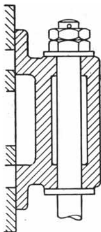
Figure 64.—Slide Valve.
