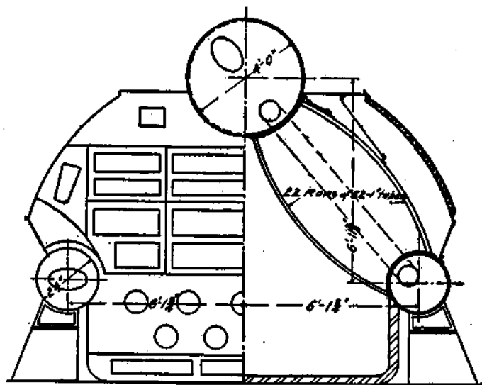
Figure 56.—White-Foster Water-Tube Boiler.
