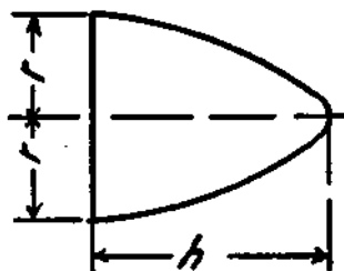
Figure 9 Paraboloid
