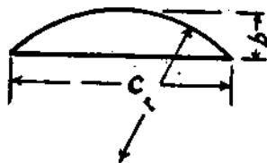
Figure 5 Spherical Segment
