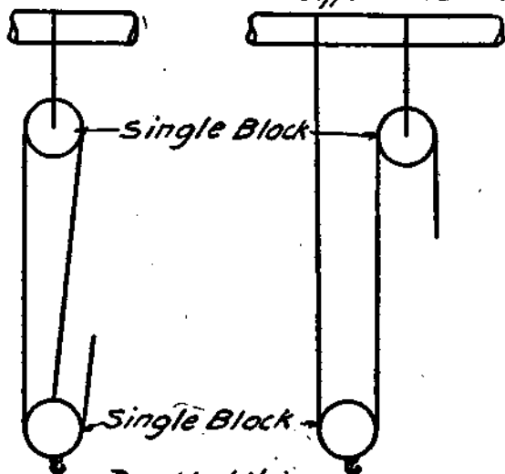
Double Whip
