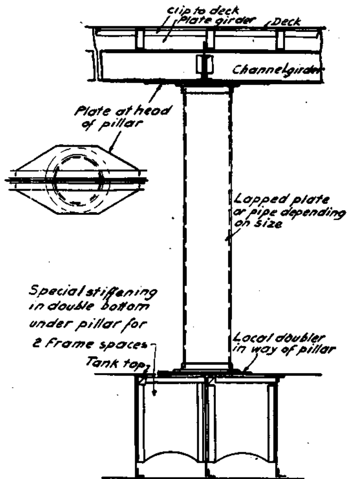
Figure 45.—Hold Pillar.
