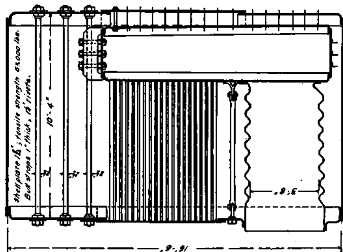
Figure 53.—Scotch Boiler.
