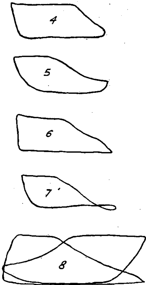
Figure 70.—Indicator Cards.
