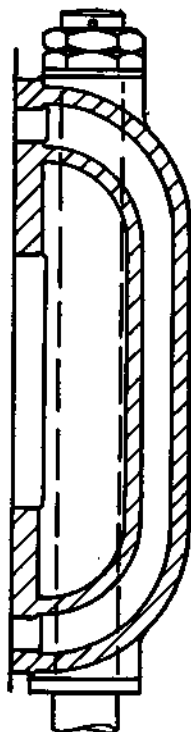
Figure 66.—Allan's Valve.
