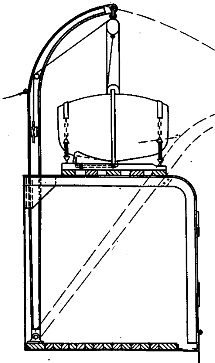
Figure 113.—Pivoted Davit. 675
