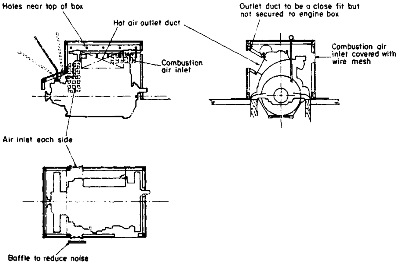
ENGINE BOX INSTALLATION
