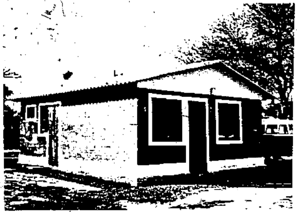
PROTOTYPE "A" : CTA's demonstration low-cost house of soil-cement blocks, built on the campus of the Catholic University, Asunción.
