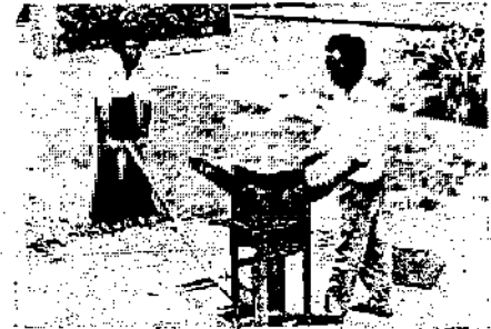
Plate-4. Ejection of soil block.
