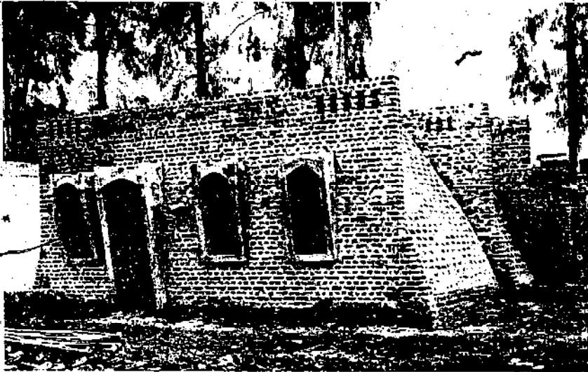
"Sarvatagriha" : An experimental low-cost vaulted house built without cement or steel and using no formwork
