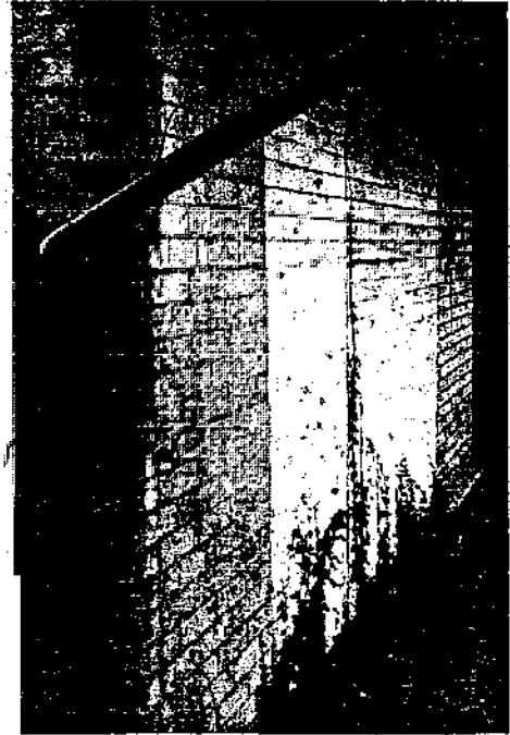
Detail view of the experimental soil-cement building, showing different surface treatments. The front corner has left untreated, but wall is in relatively good condition after 35 years of exposure.
