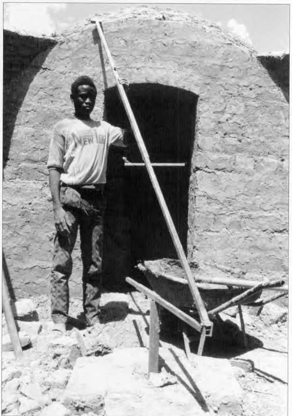
Figure 3 An adjustable radial arm is given to each mason at the end of his basic training, enabling him to build eccentric domes.
