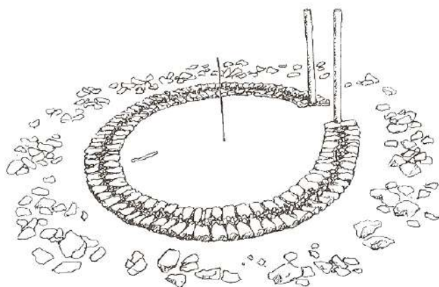
Figure 3: The first two lines of stones are laid in perfect concentric circles. Make sure that they are level, and fill the space in between with small pieces of stones
