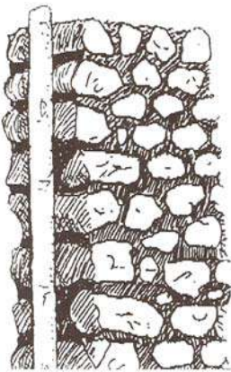
Figure 6: Try and find longer stones for the doorway, one laid across and two running back into the wall
