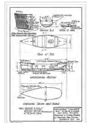
Blueprints for a concrete boat
